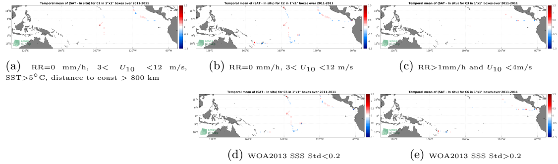
Figure 12: Temporal mean gridded over spatial boxes of size 1^{\circ}\times 1^{\circ} of \Delta SSS (Aquarius SSS L3 OR v5 - Monthly (NASA-GSFC) - TSG (GOSUD-Sailing-ship)) for 5 different subdatasets corresponding to:RR=0 mm/h, 3 < U_{10} < 12 m/s, SST >5^{\circ}\text{C} , distance to coast > 800 km (a), RR=0 mm/h, 3 < U_{10} < 12 m/s (b), RR >1 mm/h and U_{10} < 4 m/s (c), WOA2013 SSS Std <0.2 (d), WOA2013 SSS Std >0.2 (e).
