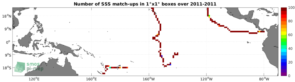
Figure 4: Number of SSS match-ups between TSG (GOSUD-Sailing-ship) SSS and the Aquarius SSS L3 OR v5 - Monthly (NASA-GSFC) SSS product for the Tropical Pacific Ocean Pi-MEP region over 1^\circ \times 1^\circ boxes and for the full satellite product period.
