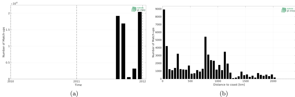
Figure 1: Number of match-ups between TSG (GOSUD-Sailing-ship) and Aquarius SSS L3 OR v5 - Monthly (NASA-GSFC) SSS as a function of time (a) and as function of the distance to coast (b) over the Tropical Pacific Ocean Pi-MEP region and for the full satellite product period.
