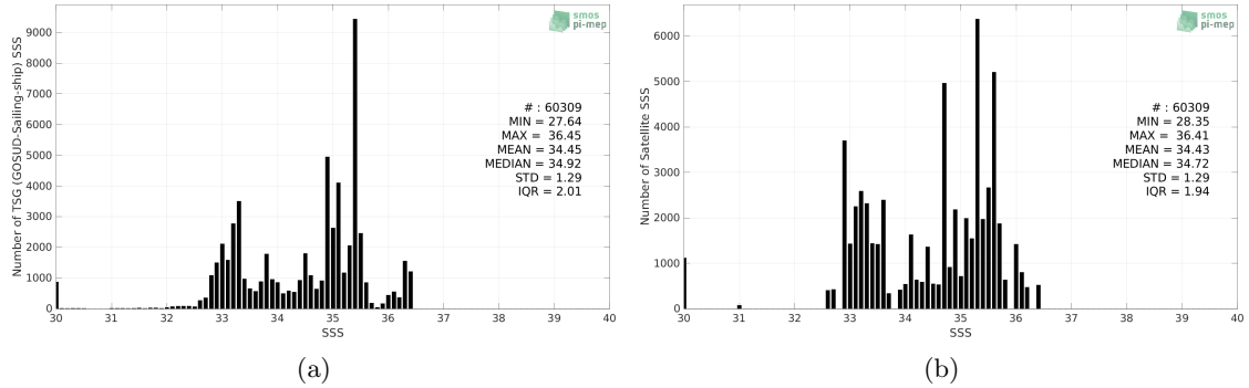
Figure 2: Histograms of SSS from TSG (GOSUD-Sailing-ship) (a) and Aquarius SSS L3 OR v5 - Monthly (NASA-GSFC) (b) considering all match-up pairs per bins of 0.1 over the Tropical Pacific Ocean Pi-MEP region and for the full satellite product period.
