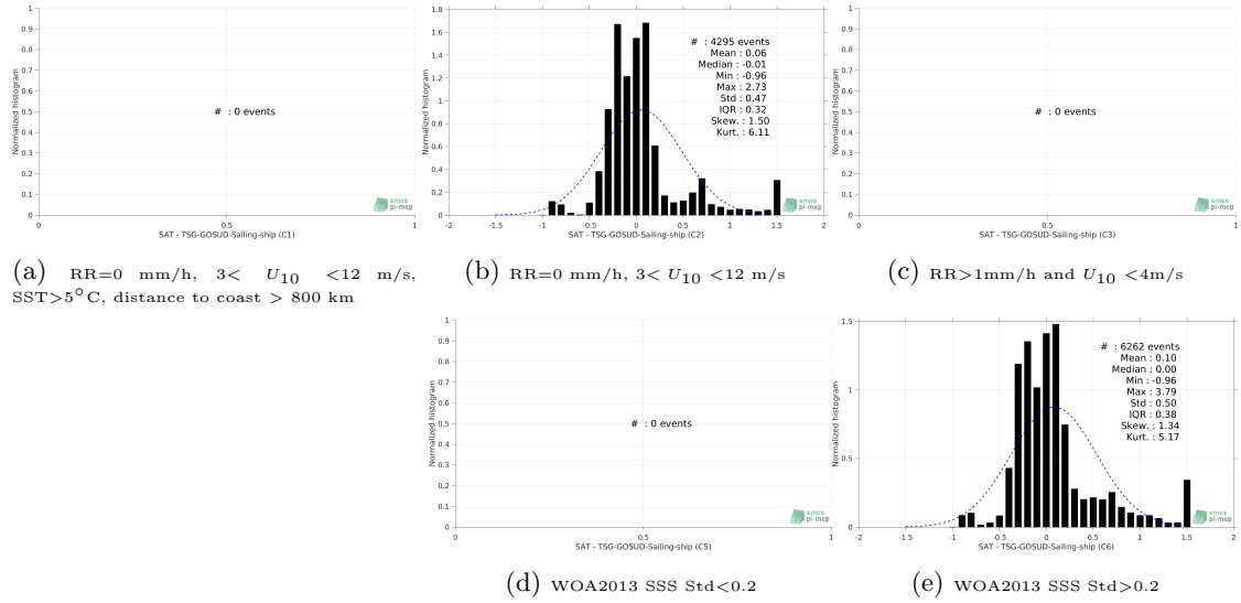
Figure 13: Normalized histogram of \Delta SSS (Aquarius-L3-OR-V5-MONTHLY-1DEG - TSG-GOSUD-Sailing-ship) for 5 different subdatasets corresponding to: RR=0 mm/h, 3 < U_{10} < 12 m/s, SST > 5°C, distance to coast > 800 km (a), RR=0 mm/h, 3 < U_{10} < 12 m/s (b), RR > 1mm/h and U_{10} < 4 m/s (c), WOA2013 SSS Std < 0.2 (d), WOA2013 SSS Std > 0.2 (e).
