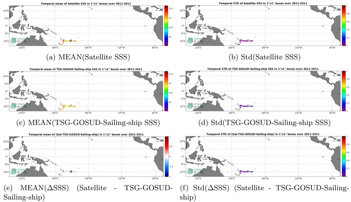
Figure 6: Temporal mean (left) and Std (right) of SSS from Aquarius-L3-OR-V5-MONTHLY-1DEG (top), TSG-GOSUD-Sailing-ship (middle), and of \Delta SSS (Satellite - TSG-GOSUD-Sailing-ship). Only match-up pairs are used to generate these maps.
