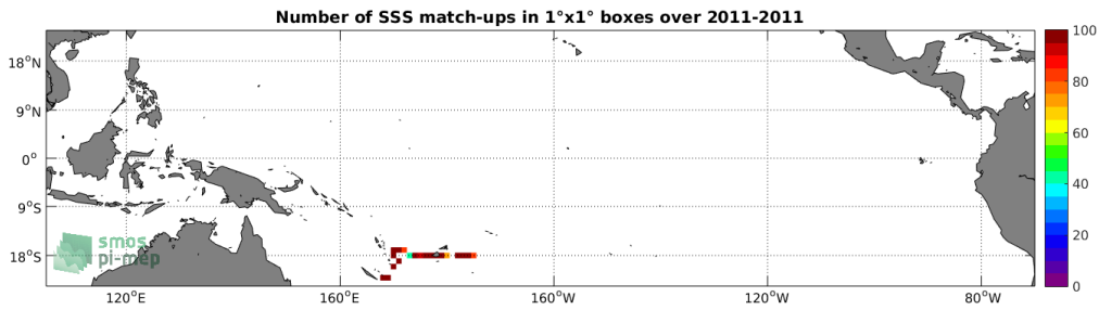
Figure 4: Number of SSS match-ups between TSG-GOSUD-Sailing-ship SSS and the Aquarius-L3-OR-V5-MONTHLY-1DEG SSS product for the Tropical Pacific Ocean Pi-MEP region over 1^\circ \times 1^\circ boxes and for the full satellite product period.
