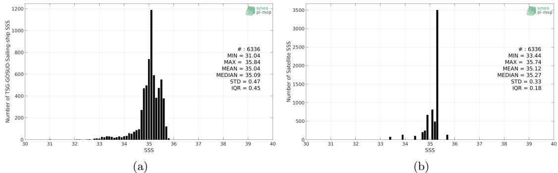
Figure 2: Histograms of SSS from TSG-GOSUD-Sailing-ship (a) and Aquarius-L3-OR-V5-MONTHLY-1DEG (b) considering all match-up pairs per bins of 0.1 over the Tropical Pacific Ocean Pi-MEP region and for the full satellite product period.
