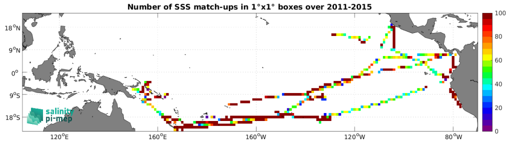
Figure 5: Number of SSS match-ups between TSG (GOSUD-Research-vessel) SSS and the Aquarius SSS L3 OR v5 - Monthly (NASA-GSFC) SSS product for the Tropical Pacific Ocean Pi-MEP region over 1^\circ \times 1^\circ boxes and for the full satellite product period.
