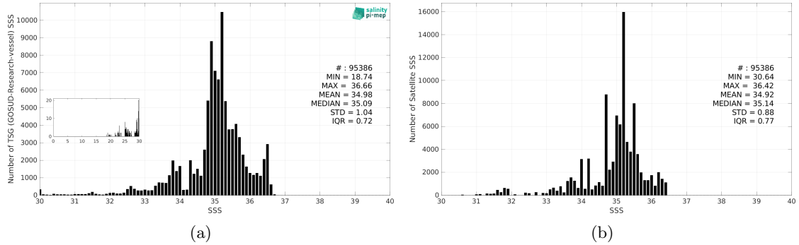
Figure 3: Histograms of SSS from TSG (GOSUD-Research-vessel) (a) and Aquarius SSS L3 OR v5 - Monthly (NASA-GSFC) (b) considering all match-up pairs per bins of 0.1 over the Tropical Pacific Ocean Pi-MEP region and for the full satellite product period.
