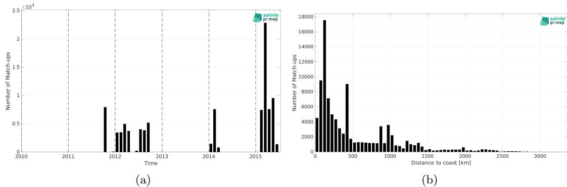
Figure 2: Number of match-ups between TSG (GOSUD-Research-vessel) and Aquarius SSS L3 OR v5 - Monthly (NASA-GSFC) SSS as a function of time (a) and as function of the distance to coast (b) over the Tropical Pacific Ocean Pi-MEP region and for the full satellite product period.
