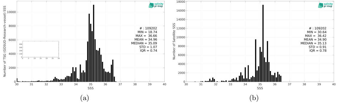
Figure 2: Histograms of SSS from TSG (GOSUD-Research-vessel) (a) and Aquarius SSS L3 OR v5 - Monthly (NASA-GSFC) (b) considering all match-up pairs per bins of 0.1 over the Tropical Pacific Ocean Pi-MEP region and for the full satellite product period.
