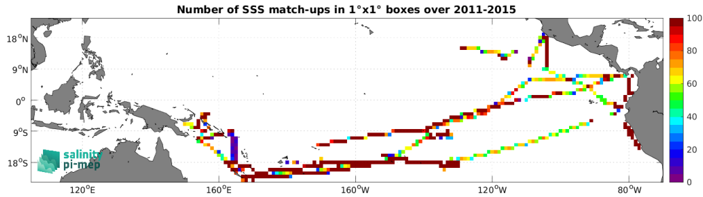
Figure 4: Number of SSS match-ups between TSG (GOSUD-Research-vessel) SSS and the Aquarius SSS L3 OR v5 - Monthly (NASA-GSFC) SSS product for the Tropical Pacific Ocean Pi-MEP region over 1^\circ \times 1^\circ boxes and for the full satellite product period.
