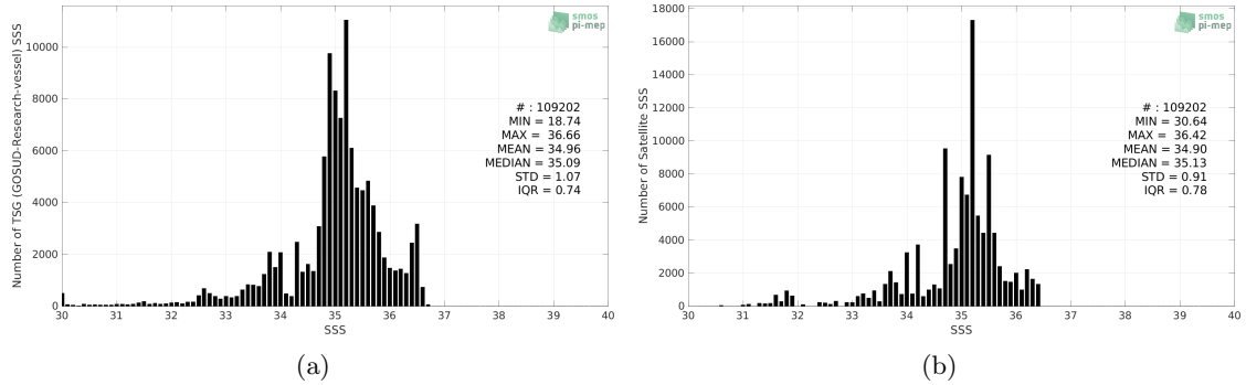
Figure 2: Histograms of SSS from TSG (GOSUD-Research-vessel) (a) and Aquarius SSS L3 OR v5 - Monthly (NASA-GSFC) (b) considering all match-up pairs per bins of 0.1 over the Tropical Pacific Ocean Pi-MEP region and for the full satellite product period.
