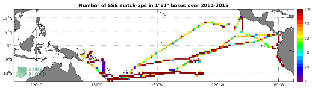
Figure 4: Number of SSS match-ups between TSG-GOSUD-Research-vessel SSS and the Aquarius-L3-OR-V5-MONTHLY-1DEG SSS product for the Tropical Pacific Ocean Pi-MEP region over 1^\circ \times 1^\circ boxes and for the full satellite product period.
