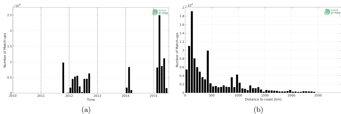
Figure 1: Number of match-ups between TSG-GOSUD-Research-vessel and Aquarius-L3-OR-V5-MONTHLY-1DEG SSS as a function of time (a) and as function of the distance to coast (b) over the Tropical Pacific Ocean Pi-MEP region and for the full satellite product period.
