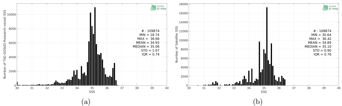
Figure 2: Histograms of SSS from TSG-GOSUD-Research-vessel (a) and Aquarius-L3-OR-V5-MONTHLY-1DEG (b) considering all match-up pairs per bins of 0.1 over the Tropical Pacific Ocean Pi-MEP region and for the full satellite product period.
