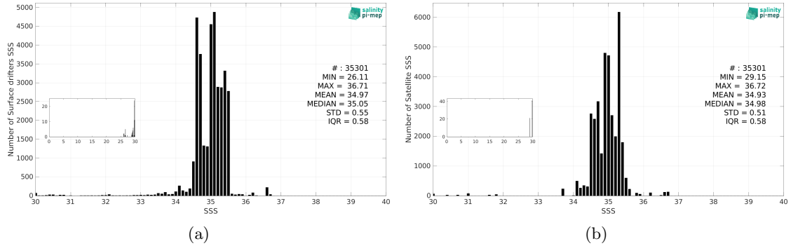
Figure 3: Histograms of SSS from Surface drifters (a) and Aquarius SSS L3 OR v5 - Monthly (NASA-GSFC) (b) considering all match-up pairs per bins of 0.1 over the Tropical Pacific Ocean Pi-MEP region and for the full satellite product period.
