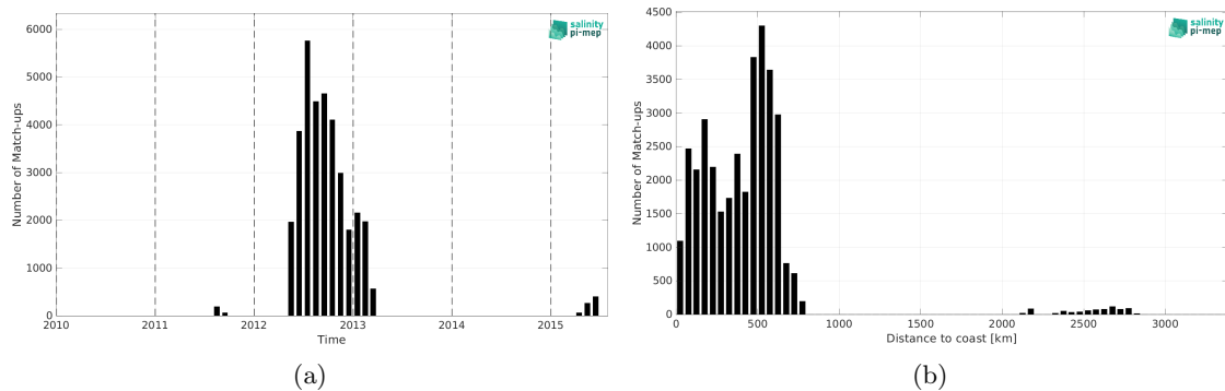
Figure 2: Number of match-ups between Surface drifters and Aquarius SSS L3 OR v5 - Monthly (NASA-GSFC) SSS as a function of time (a) and as function of the distance to coast (b) over the Tropical Pacific Ocean Pi-MEP region and for the full satellite product period.
