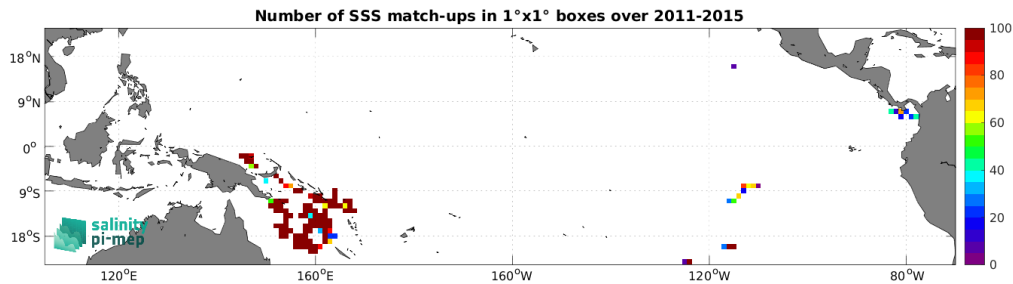
Figure 4: Number of SSS match-ups between Surface drifters SSS and the Aquarius SSS L3 OR v5 - Monthly (NASA-GSFC) SSS product for the Tropical Pacific Ocean Pi-MEP region over 1^\circ \times 1^\circ boxes and for the full satellite product period.
