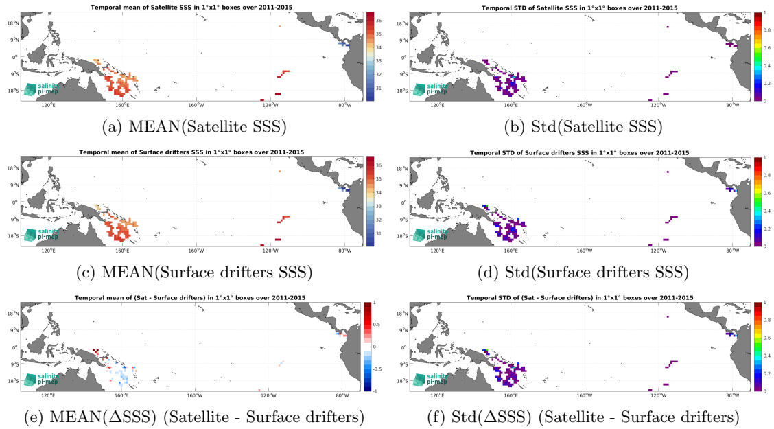
Figure 6: Temporal mean (left) and Std (right) of SSS from Aquarius SSS L3 OR v5 - Monthly (NASA-GSFC) (top), Surface drifters (middle), and of \Delta SSS (Satellite - Surface drifters). Only match-up pairs are used to generate these maps.
