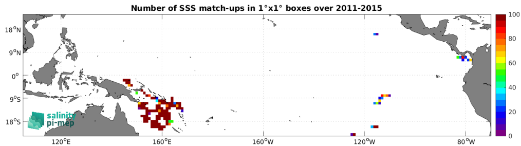
Figure 3: Number of SSS match-ups between Surface drifters SSS and the Aquarius SSS L3 OR v5 - Monthly (NASA-GSFC) SSS product for the Tropical Pacific Ocean Pi-MEP region over 1^\circ \times 1^\circ boxes and for the full satellite product period.
