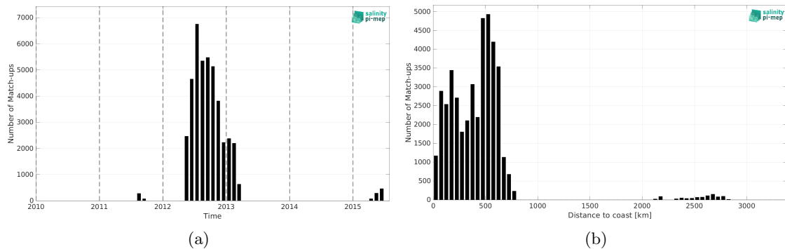
Figure 1: Number of match-ups between Surface drifters and Aquarius SSS L3 OR v5 - Monthly (NASA-GSFC) SSS as a function of time (a) and as function of the distance to coast (b) over the Tropical Pacific Ocean Pi-MEP region and for the full satellite product period.
