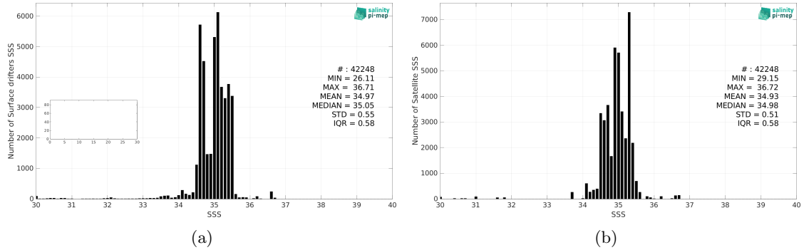
Figure 2: Histograms of SSS from Surface drifters (a) and Aquarius SSS L3 OR v5 - Monthly (NASA-GSFC) (b) considering all match-up pairs per bins of 0.1 over the Tropical Pacific Ocean Pi-MEP region and for the full satellite product period.
