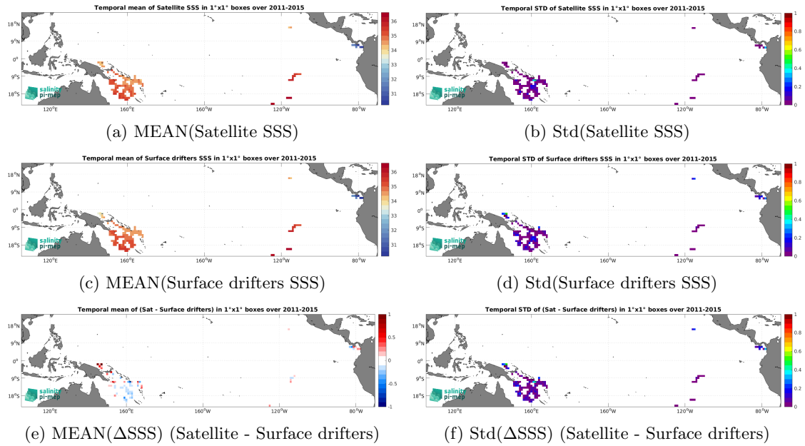
Figure 5: Temporal mean (left) and Std (right) of SSS from Aquarius SSS L3 OR v5 - Monthly (NASA-GSFC) (top), Surface drifters (middle), and of \Delta SSS (Satellite - Surface drifters). Only match-up pairs are used to generate these maps.
