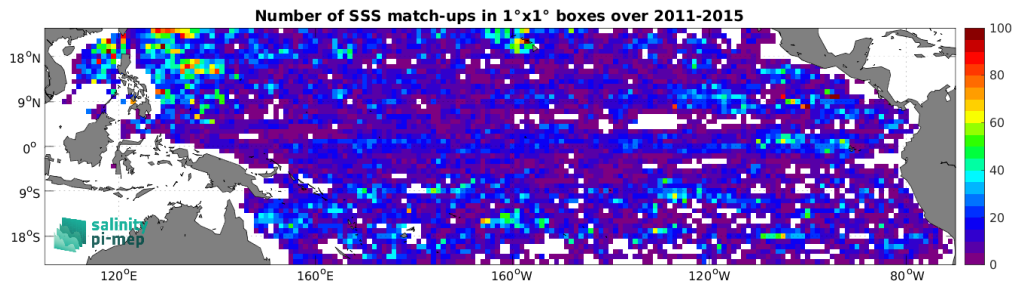
Figure 5: Number of SSS match-ups between Argo SSS and the Aquarius SSS L3 OR v5 - Monthly (NASA-GSFC) SSS product for the Tropical Pacific Ocean Pi-MEP region over 1^\circ \times 1^\circ boxes and for the full satellite product period.
