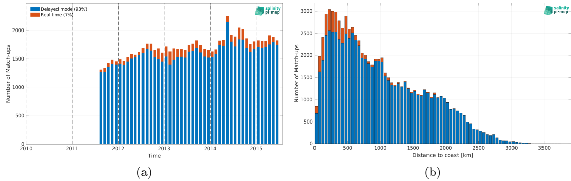
Figure 2: Number of match-ups between Argo and Aquarius SSS L3 OR v5 - Monthly (NASA-GSFC) SSS as a function of time (a) and as function of the distance to coast (b) over the Tropical Pacific Ocean Pi-MEP region and for the full satellite product period.
