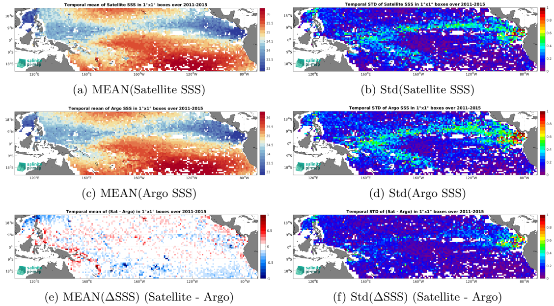
Figure 7: Temporal mean (left) and Std (right) of SSS from Aquarius SSS L3 OR v5 - Monthly (NASA-GSFC) (top), Argo (middle), and of \Delta SSS (Satellite - Argo). Only match-up pairs are used to generate these maps.
