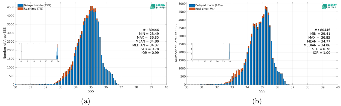
Figure 3: Histograms of SSS from Argo (a) and Aquarius SSS L3 OR v5 - Monthly (NASA-GSFC) (b) considering all match-up pairs per bins of 0.1 over the Tropical Pacific Ocean Pi-MEP region and for the full satellite product period.
