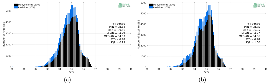
Figure 2: Histograms of SSS from Argo (a) and Aquarius-L3-OR-V5-MONTHLY-1DEG (b) considering all match-up pairs per bins of 0.1 over the Tropical Pacific Ocean Pi-MEP region and for the full satellite product period.
