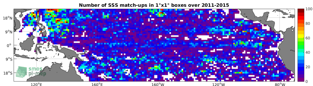
Figure 4: Number of SSS match-ups between Argo SSS and the Aquarius-L3-OR-V5-MONTHLY-1DEG SSS product for the Tropical Pacific Ocean Pi-MEP region over 1°x1° boxes and for the full satellite product period.
