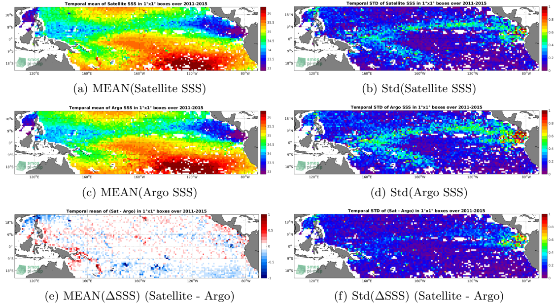
Figure 6: Temporal mean (left) and Std (right) of SSS from Aquarius-L3-OR-V5-MONTHLY-1DEG (top), Argo (middle), and of \Delta SSS (Satellite - Argo). Only match-up pairs are used to generate these maps.
