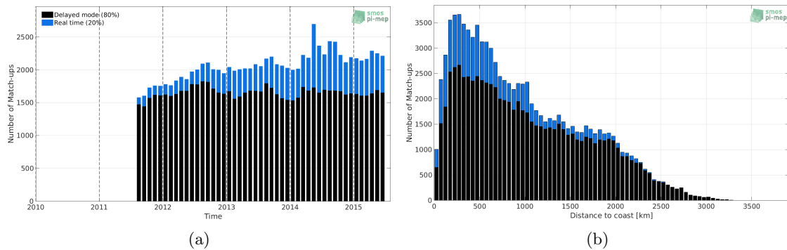
Figure 1: Number of match-ups between Argo and Aquarius-L3-OR-V5-MONTHLY-1DEG SSS as a function of time (a) and as function of the distance to coast (b) over the Tropical Pacific Ocean Pi-MEP region and for the full satellite product period.
