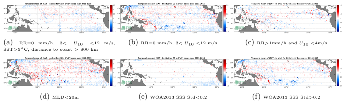
Figure 12: Temporal mean gridded over spatial boxes of size 1^\circ \times 1^\circ of \Delta SSS (Aquarius-L3-OR-V5-MONTHLY-1DEG - Argo) for 6 different subdatasets corresponding to:RR=0 mm/h, 3 < U_{10} < 12 m/s, SST >5^\circ\text{C} , distance to coast > 800 km (a), RR=0 mm/h, 3 < U_{10} < 12 m/s (b), RR >1 mm/h and U_{10} < 4 m/s (c),MLD <20 m (d),WOA2013 SSS Std <0.2 (e),WOA2013 SSS Std >0.2 (f).
