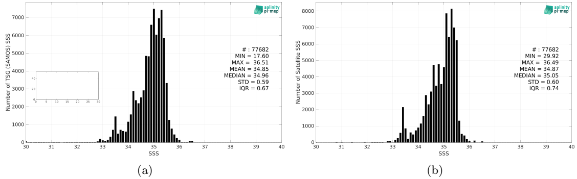
Figure 2: Histograms of SSS from TSG (SAMOS) (a) and Aquarius SSS L3 OR v5 - Monthly - Rain mask (NASA-GSFC) (b) considering all match-up pairs per bins of 0.1 over the Tropical Pacific Ocean Pi-MEP region and for the full satellite product period.
