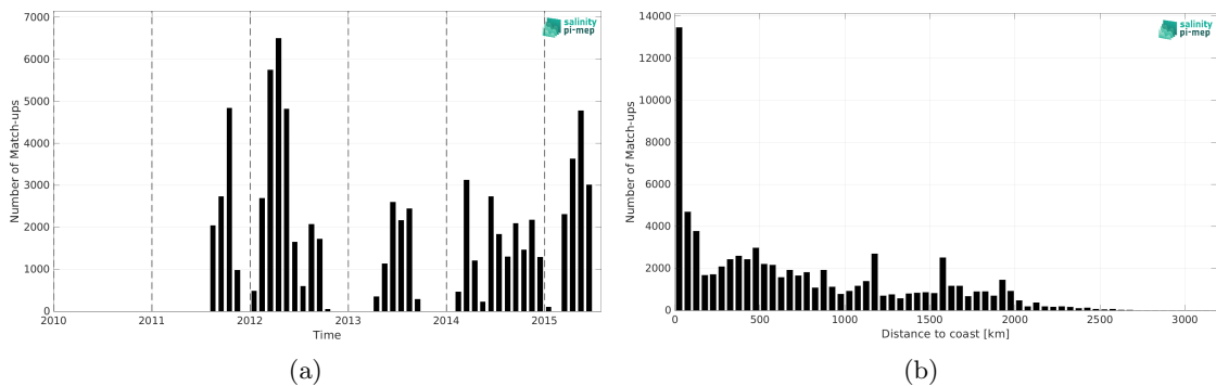
Figure 1: Number of match-ups between TSG (SAMOS) and Aquarius SSS L3 OR v5 - Monthly - Rain mask (NASA-GSFC) SSS as a function of time (a) and as function of the distance to coast (b) over the Tropical Pacific Ocean Pi-MEP region and for the full satellite product period.
