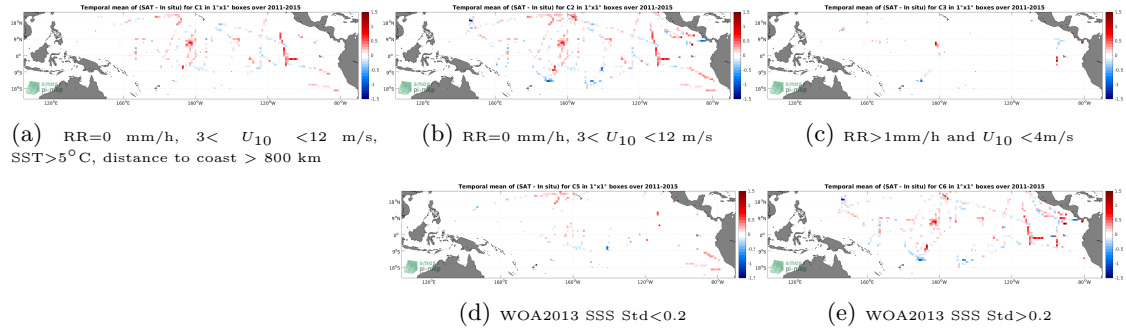
Figure 12: Temporal mean gridded over spatial boxes of size 1^{\circ}\times 1^{\circ} of \Delta\text{SSS} (Aquarius SSS L3 OR v5 - Monthly - Rain mask (NASA-GSFC) - TSG (SAMOS)) for 5 different subdatasets corresponding to:RR=0 mm/h, 3 < U_{10} < 12 m/s, SST >5^{\circ}\text{C} , distance to coast > 800 km (a), RR=0 mm/h, 3 < U_{10} < 12 m/s (b), RR >1 mm/h and U_{10} < 4 m/s (c), WOA2013 SSS Std <0.2 (d), WOA2013 SSS Std >0.2 (e).
