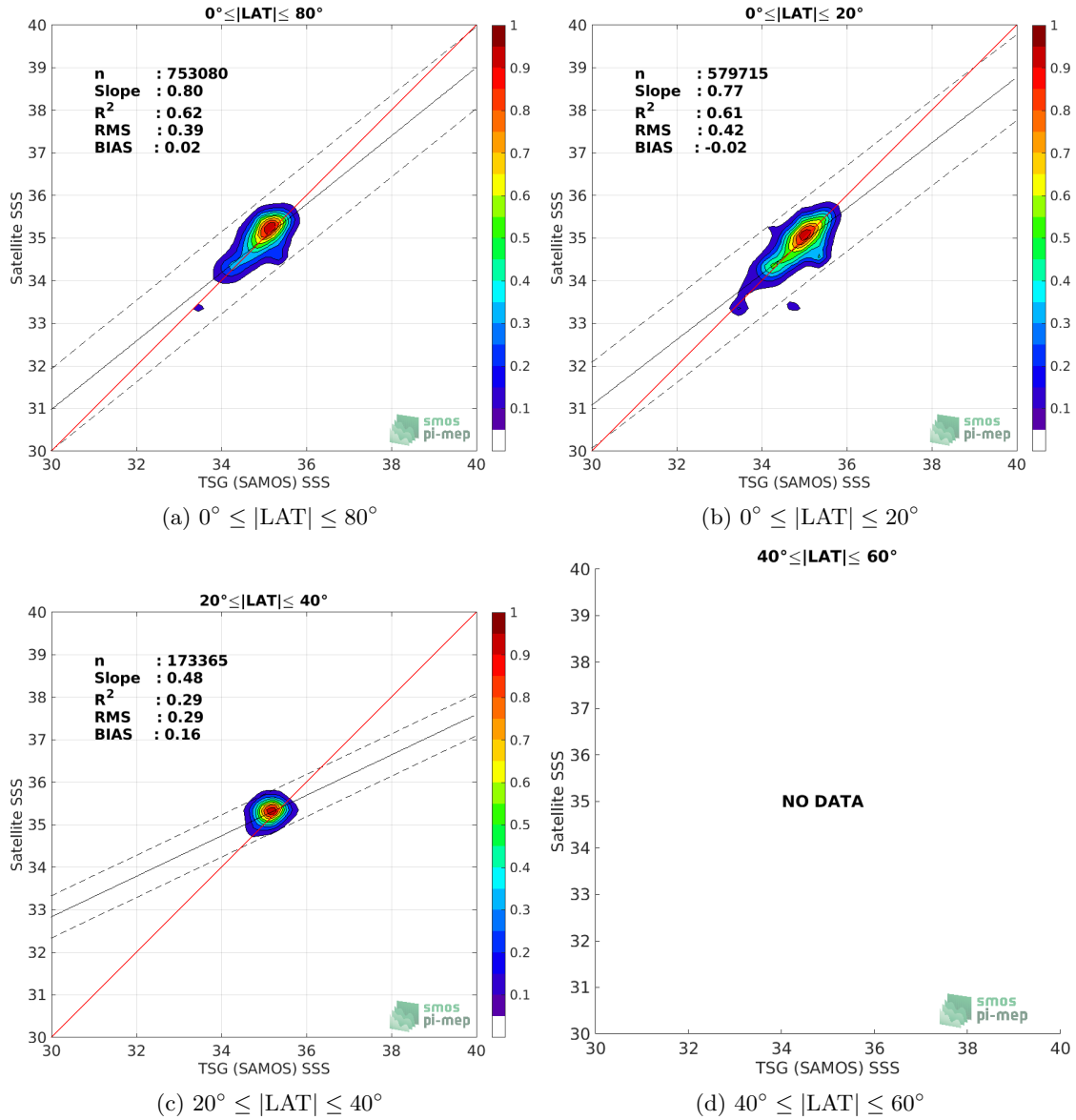
Figure 9: Contour maps of the concentration of Aquarius SSS L3 OR v5 - Monthly - Rain mask (NASA-GSFC) SSS ( y -axis) versus TSG (SAMOS) SSS ( x -axis) at match-up pairs for different latitude bands. For each plot, the red line shows x=y . The black thin and dashed lines indicate a linear fit through the data cloud and the \pm 95\% confidence levels, respectively. The number match-up pairs n , the slope and R^2 coefficient of the linear fit, the root mean square (RMS) and the mean bias between satellite and in situ data are indicated for each latitude band in each plots.
