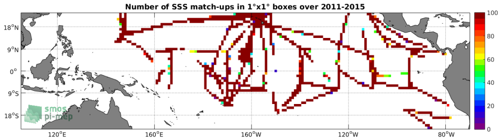
Figure 4: Number of SSS match-ups between TSG-SAMOS SSS and the Aquarius-L3-OR-V5-MONTHLY-RAIN-MASK-1DEG SSS product for the Tropical Pacific Ocean Pi-MEP region over 1^\circ \times 1^\circ boxes and for the full satellite product period.
