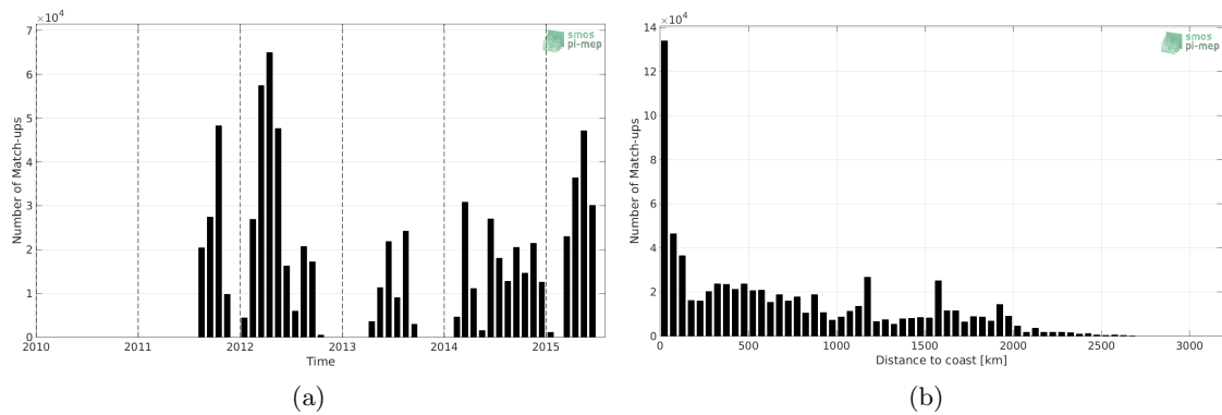
Figure 1: Number of match-ups between TSG-SAMOS and Aquarius-L3-OR-V5-MONTHLY-RAIN-MASK-1DEG SSS as a function of time (a) and as function of the distance to coast (b) over the Tropical Pacific Ocean Pi-MEP region and for the full satellite product period.
