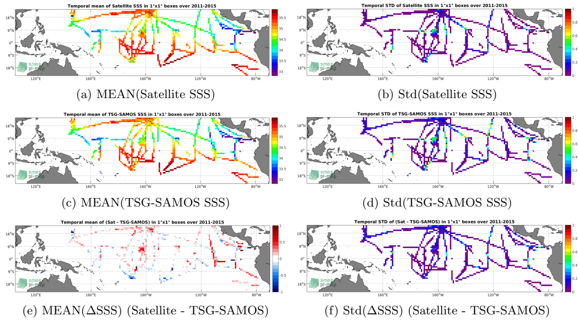
Figure 6: Temporal mean (left) and Std (right) of SSS from Aquarius-L3-OR-V5-MONTHLY-RAIN-MASK-1DEG (top), TSG-SAMOS (middle), and of \Delta SSS (Satellite - TSG-SAMOS). Only match-up pairs are used to generate these maps.
