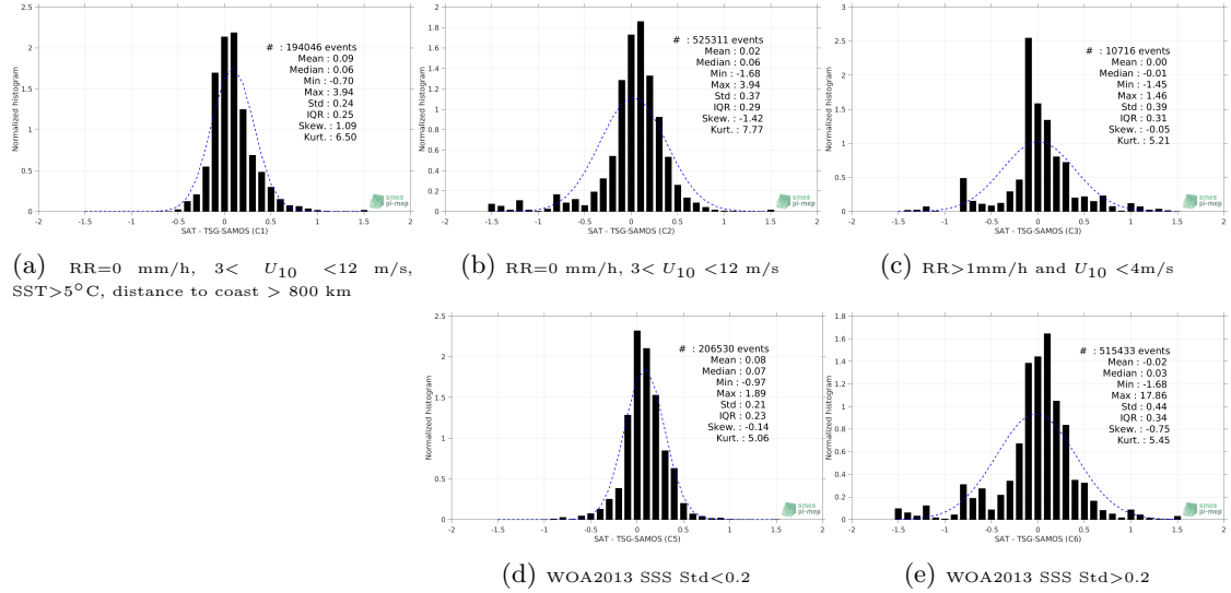
Figure 13: Normalized histogram of \Delta\text{SSS} (Aquarius-L3-OR-V5-MONTHLY-RAIN-MASK-1DEG - TSG-SAMOS) for 5 different subdatasets corresponding to: RR=0 mm/h, 3 < U_{10} < 12 m/s, SST > 5^\circ\text{C} , distance to coast > 800 km (a), RR=0 mm/h, 3 < U_{10} < 12 m/s (b), RR > 1 mm/h and U_{10} < 4 m/s (c), WOA2013 SSS Std < 0.2 (d), WOA2013 SSS Std > 0.2 (e).
