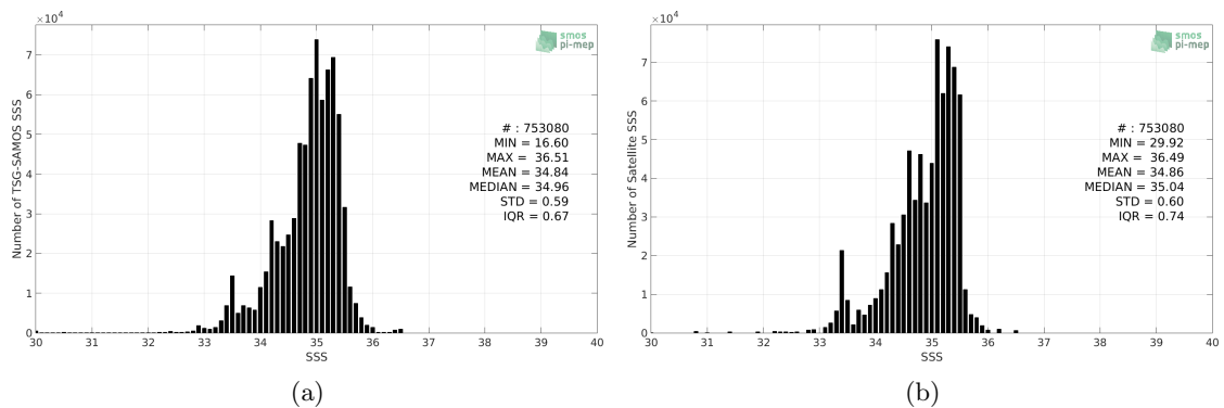
Figure 2: Histograms of SSS from TSG-SAMOS (a) and Aquarius-L3-OR-V5-MONTHLY-RAIN-MASK-1DEG (b) considering all match-up pairs per bins of 0.1 over the Tropical Pacific Ocean Pi-MEP region and for the full satellite product period.
