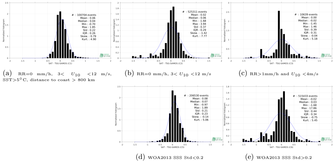
Figure 13: Normalized histogram of \Delta SSS (Aquarius-L3-OR-V5-MONTHLY-RAIN-MASK-1DEG - TSG-SAMOS) for 5 different subdatasets corresponding to: RR=0 mm/h, 3 < U_{10} < 12 m/s, SST >5^\circ C, distance to coast > 800 km (a), RR=0 mm/h, 3 < U_{10} < 12 m/s (b), RR >1 mm/h and U_{10} < 4 m/s (c), WOA2013 SSS Std <0.2 (d), WOA2013 SSS Std >0.2 (e).
