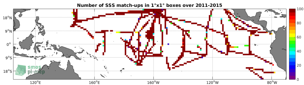
Figure 4: Number of SSS match-ups between TSG-SAMOS SSS and the Aquarius-L3-OR-V5-MONTHLY-RAIN-MASK-1DEG SSS product for the Tropical Pacific Ocean Pi-MEP region over 1^\circ \times 1^\circ boxes and for the full satellite product period.
