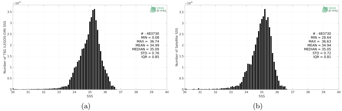
Figure 2: Histograms of SSS from TSG (LEGOS-DM) (a) and Aquarius SSS L3 OR v5 - Monthly - Rain mask (NASA-GSFC) (b) considering all match-up pairs per bins of 0.1 over the Tropical Pacific Ocean Pi-MEP region and for the full satellite product period.
