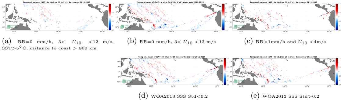
Figure 12: Temporal mean gridded over spatial boxes of size 1^{\circ}\times 1^{\circ} of \Delta\text{SSS} (Aquarius SSS L3 OR v5 - Monthly - Rain mask (NASA-GSFC) - TSG (LEGOS-DM)) for 5 different subdatasets corresponding to:RR=0 mm/h, 3 < U_{10} < 12 m/s, SST > 5^{\circ}\text{C} , distance to coast > 800 km (a), RR=0 mm/h, 3 < U_{10} < 12 m/s (b), RR > 1 mm/h and U_{10} < 4 m/s (c), WOA2013 SSS Std < 0.2 (d), WOA2013 SSS Std > 0.2 (e).
