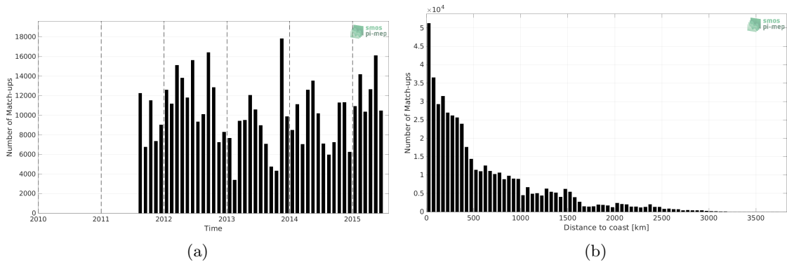
Figure 1: Number of match-ups between TSG (LEGOS-DM) and Aquarius SSS L3 OR v5 - Monthly - Rain mask (NASA-GSFC) SSS as a function of time (a) and as function of the distance to coast (b) over the Tropical Pacific Ocean Pi-MEP region and for the full satellite product period.
