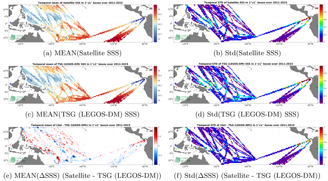
Figure 6: Temporal mean (left) and Std (right) of SSS from Aquarius SSS L3 OR v5 - Monthly - Rain mask (NASA-GSFC) (top), TSG (LEGOS-DM) (middle), and of \Delta SSS (Satellite - TSG (LEGOS-DM)). Only match-up pairs are used to generate these maps.
