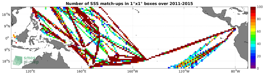
Figure 4: Number of SSS match-ups between TSG (LEGOS-DM) SSS and the Aquarius SSS L3 OR v5 - Monthly - Rain mask (NASA-GSFC) SSS product for the Tropical Pacific Ocean Pi-MEP region over 1^\circ \times 1^\circ boxes and for the full satellite product period.
