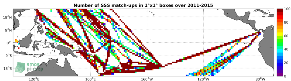
Figure 4: Number of SSS match-ups between TSG-LEGOS-DM SSS and the Aquarius-L3-OR-V5-MONTHLY-RAIN-MASK-1DEG SSS product for the Tropical Pacific Ocean Pi-MEP region over 1^\circ \times 1^\circ boxes and for the full satellite product period.
