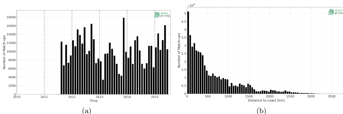
Figure 1: Number of match-ups between TSG-LEGOS-DM and Aquarius-L3-OR-V5-MONTHLY-RAIN-MASK-1DEG SSS as a function of time (a) and as function of the distance to coast (b) over the Tropical Pacific Ocean Pi-MEP region and for the full satellite product period.
