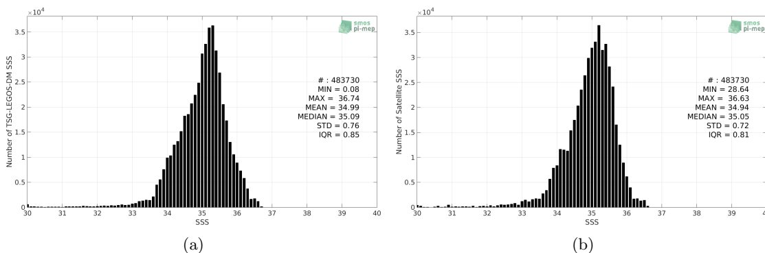
Figure 2: Histograms of SSS from TSG-LEGOS-DM (a) and Aquarius-L3-OR-V5-MONTHLY-RAIN-MASK-1DEG (b) considering all match-up pairs per bins of 0.1 over the Tropical Pacific Ocean Pi-MEP region and for the full satellite product period.
