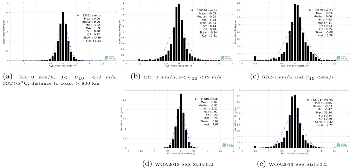
Figure 13: Normalized histogram of \Delta SSS (Aquarius-L3-OR-V5-MONTHLY-RAIN-MASK-1DEG - TSG-LEGOS-DM) for 5 different subdatasets corresponding to: RR=0 mm/h, 3 < U_{10} < 12 m/s, SST >5^\circ C, distance to coast > 800 km (a), RR=0 mm/h, 3 < U_{10} < 12 m/s (b), RR >1 mm/h and U_{10} < 4 m/s (c), WOA2013 SSS Std <0.2 (d), WOA2013 SSS Std >0.2 (e).
