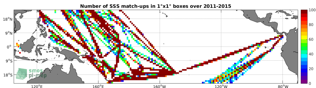
Figure 4: Number of SSS match-ups between TSG-LEGOS-DM SSS and the Aquarius-L3-OR-V5-MONTHLY-RAIN-MASK-1DEG SSS product for the Tropical Pacific Ocean Pi-MEP region over 1^\circ \times 1^\circ boxes and for the full satellite product period.
