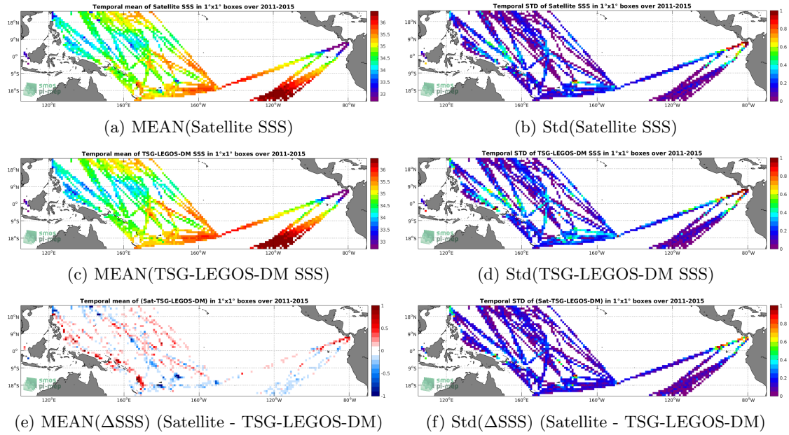
Figure 6: Temporal mean (left) and Std (right) of SSS from Aquarius-L3-OR-V5-MONTHLY-RAIN-MASK-1DEG (top), TSG-LEGOS-DM (middle), and of \Delta SSS (Satellite - TSG-LEGOS-DM). Only match-up pairs are used to generate these maps.
