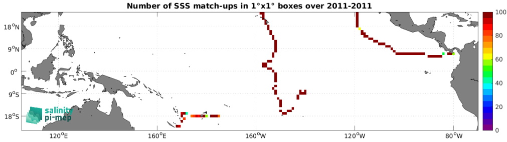
Figure 5: Number of SSS match-ups between TSG (GOSUD-Sailing-ship) SSS and the Aquarius SSS L3 OR v5 - Monthly - Rain mask (NASA-GSFC) SSS product for the Tropical Pacific Ocean Pi-MEP region over 1^\circ \times 1^\circ boxes and for the full satellite product period.
