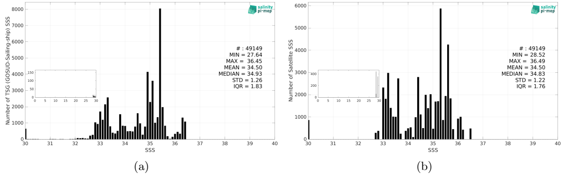
Figure 3: Histograms of SSS from TSG (GOSUD-Sailing-ship) (a) and Aquarius SSS L3 OR v5 - Monthly - Rain mask (NASA-GSFC) (b) considering all match-up pairs per bins of 0.1 over the Tropical Pacific Ocean Pi-MEP region and for the full satellite product period.
