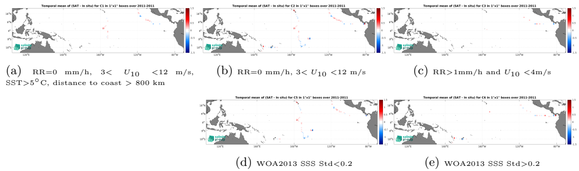
Figure 12: Temporal mean gridded over spatial boxes of size 1^{\circ}\times 1^{\circ} of \Delta SSS (Aquarius SSS L3 OR v5 - Monthly - Rain mask (NASA-GSFC) - TSG (GOSUD-Sailing-ship)) for 5 different subdatasets corresponding to:RR=0 mm/h, 3 < U_{10} < 12 m/s, SST >5^{\circ}\text{C} , distance to coast > 800 km (a), RR=0 mm/h, 3 < U_{10} < 12 m/s (b), RR >1 mm/h and U_{10} < 4 m/s (c), WOA2013 SSS Std <0.2 (d), WOA2013 SSS Std >0.2 (e).
