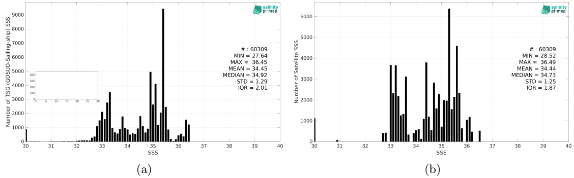
Figure 2: Histograms of SSS from TSG (GOSUD-Sailing-ship) (a) and Aquarius SSS L3 OR v5 - Monthly - Rain mask (NASA-GSFC) (b) considering all match-up pairs per bins of 0.1 over the Tropical Pacific Ocean Pi-MEP region and for the full satellite product period.
