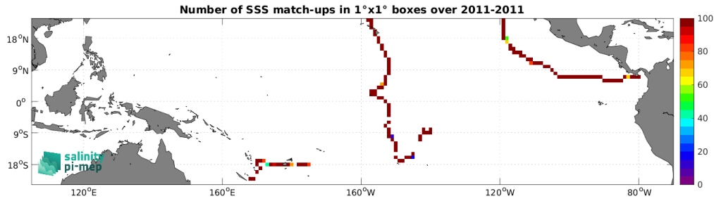
Figure 4: Number of SSS match-ups between TSG (GOSUD-Sailing-ship) SSS and the Aquarius SSS L3 OR v5 - Monthly - Rain mask (NASA-GSFC) SSS product for the Tropical Pacific Ocean Pi-MEP region over 1^\circ \times 1^\circ boxes and for the full satellite product period.
