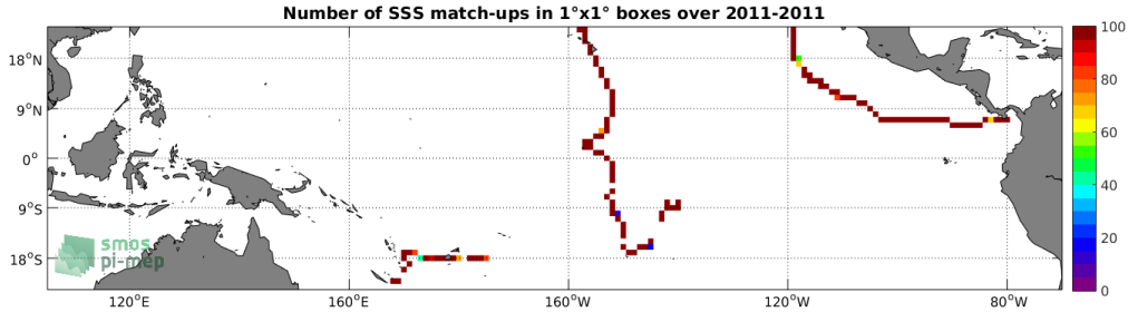
Figure 4: Number of SSS match-ups between TSG (GOSUD-Sailing-ship) SSS and the Aquarius SSS L3 OR v5 - Monthly - Rain mask (NASA-GSFC) SSS product for the Tropical Pacific Ocean Pi-MEP region over 1^\circ \times 1^\circ boxes and for the full satellite product period.
