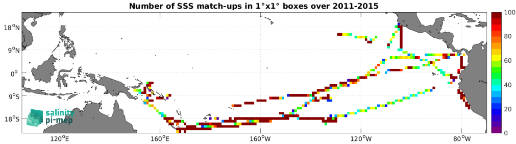
Figure 5: Number of SSS match-ups between TSG (GOSUD-Research-vessel) SSS and the Aquarius SSS L3 OR v5 - Monthly - Rain mask (NASA-GSFC) SSS product for the Tropical Pacific Ocean Pi-MEP region over 1^\circ \times 1^\circ boxes and for the full satellite product period.
