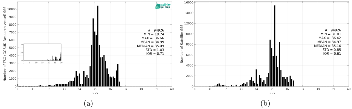
Figure 3: Histograms of SSS from TSG (GOSUD-Research-vessel) (a) and Aquarius SSS L3 OR v5 - Monthly - Rain mask (NASA-GSFC) (b) considering all match-up pairs per bins of 0.1 over the Tropical Pacific Ocean Pi-MEP region and for the full satellite product period.
