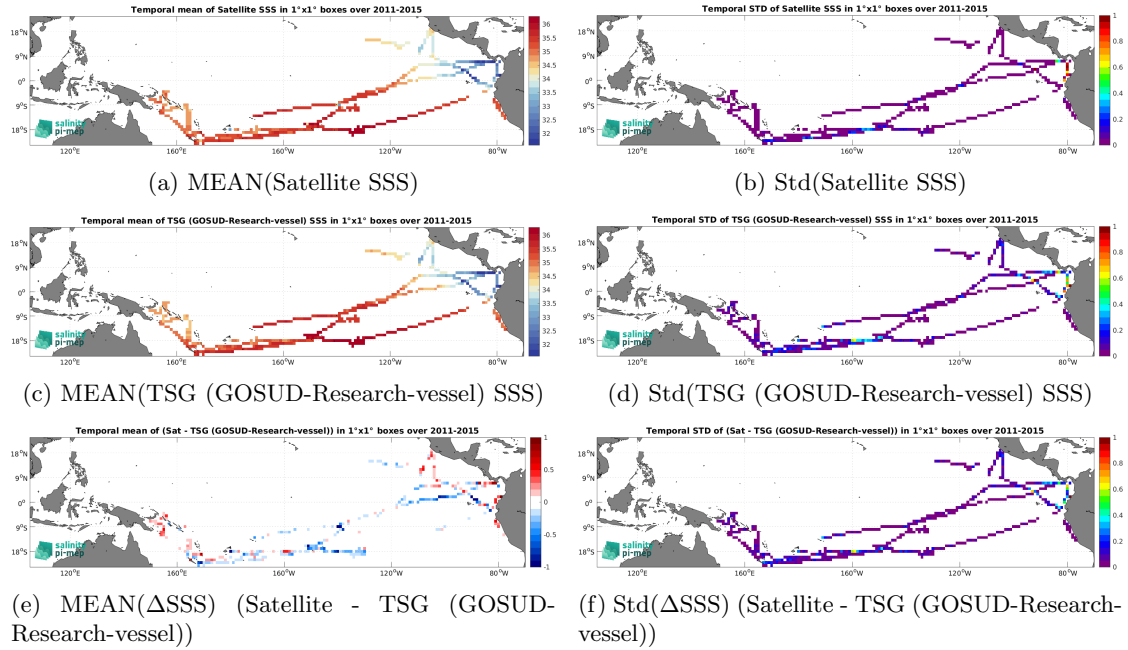
Figure 6: Temporal mean (left) and Std (right) of SSS from Aquarius SSS L3 OR v5 - Monthly - Rain mask (NASA-GSFC) (top), TSG (GOSUD-Research-vessel) (middle), and of \Delta SSS (Satellite - TSG (GOSUD-Research-vessel)). Only match-up pairs are used to generate these maps.
