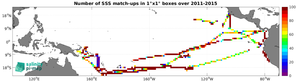
Figure 4: Number of SSS match-ups between TSG (GOSUD-Research-vessel) SSS and the Aquarius SSS L3 OR v5 - Monthly - Rain mask (NASA-GSFC) SSS product for the Tropical Pacific Ocean Pi-MEP region over 1^\circ \times 1^\circ boxes and for the full satellite product period.
