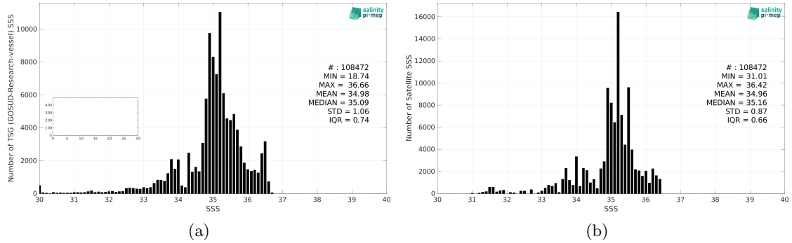
Figure 2: Histograms of SSS from TSG (GOSUD-Research-vessel) (a) and Aquarius SSS L3 OR v5 - Monthly - Rain mask (NASA-GSFC) (b) considering all match-up pairs per bins of 0.1 over the Tropical Pacific Ocean Pi-MEP region and for the full satellite product period.
