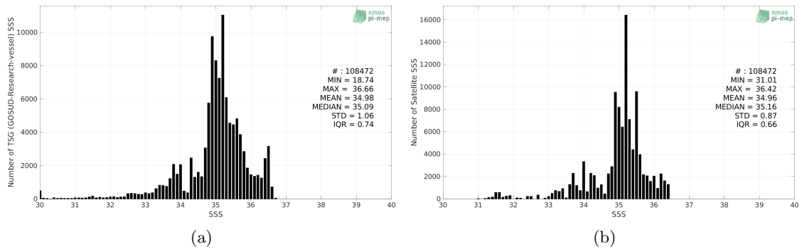
Figure 2: Histograms of SSS from TSG (GOSUD-Research-vessel) (a) and Aquarius SSS L3 OR v5 - Monthly - Rain mask (NASA-GSFC) (b) considering all match-up pairs per bins of 0.1 over the Tropical Pacific Ocean Pi-MEP region and for the full satellite product period.
