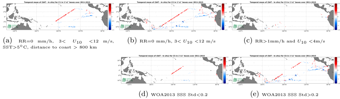
Figure 12: Temporal mean gridded over spatial boxes of size 1^\circ \times 1^\circ of \Delta SSS (Aquarius-L3-OR-V5-MONTHLY-RAIN-MASK-1DEG - TSG-GOSUD-Research-vessel) for 5 different subdatasets corresponding to: RR=0 mm/h, 3 < U_{10} < 12 m/s, SST >5^\circ\text{C} , distance to coast > 800 km (a), RR=0 mm/h, 3 < U_{10} < 12 m/s (b), RR >1 mm/h and U_{10} < 4 m/s (c), WOA2013 SSS Std <0.2 (d), WOA2013 SSS Std >0.2 (e).
