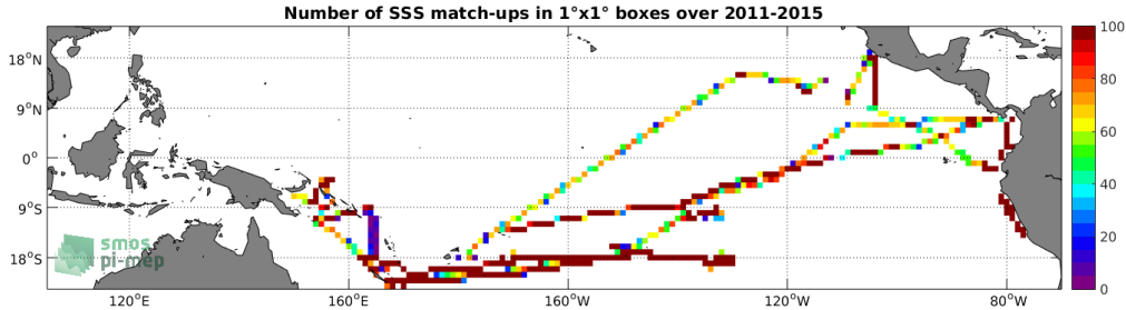
Figure 4: Number of SSS match-ups between TSG-GOSUD-Research-vessel SSS and the Aquarius-L3-OR-V5-MONTHLY-RAIN-MASK-1DEG SSS product for the Tropical Pacific Ocean Pi-MEP region over 1^\circ \times 1^\circ boxes and for the full satellite product period.
