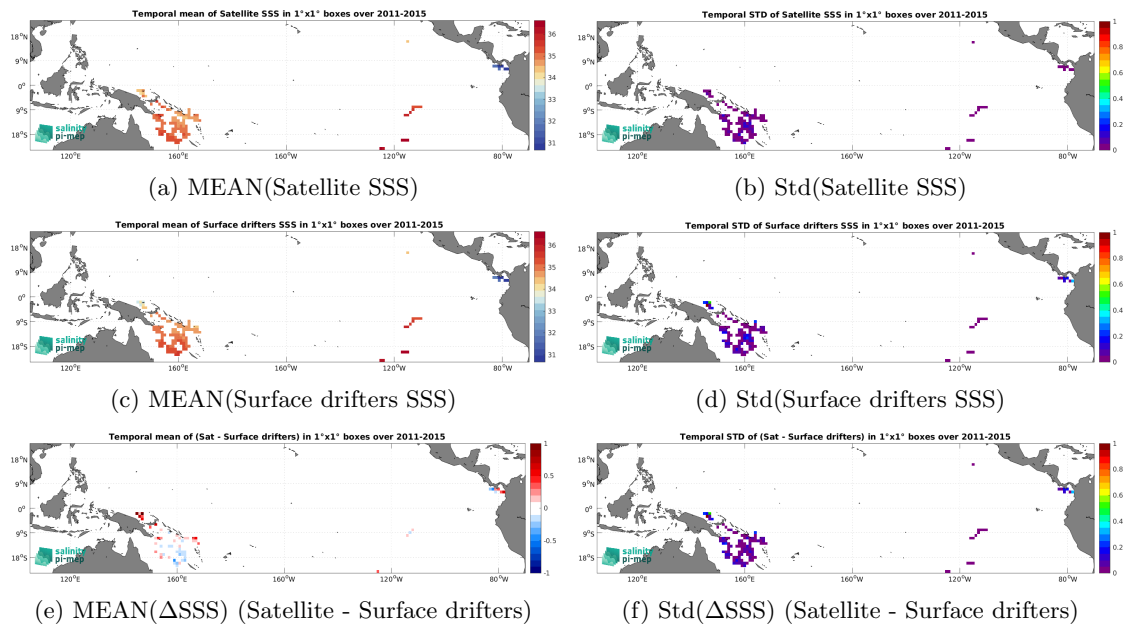
Figure 6: Temporal mean (left) and Std (right) of SSS from Aquarius SSS L3 OR v5 - Monthly - Rain mask (NASA-GSFC) (top), Surface drifters (middle), and of \Delta SSS (Satellite - Surface drifters). Only match-up pairs are used to generate these maps.
