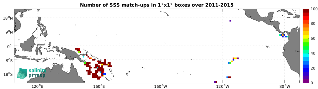
Figure 4: Number of SSS match-ups between Surface drifters SSS and the Aquarius SSS L3 OR v5 - Monthly - Rain mask (NASA-GSFC) SSS product for the Tropical Pacific Ocean Pi-MEP region over 1^\circ \times 1^\circ boxes and for the full satellite product period.
