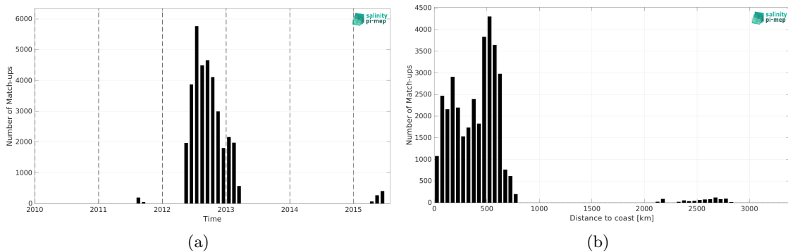
Figure 2: Number of match-ups between Surface drifters and Aquarius SSS L3 OR v5 - Monthly - Rain mask (NASA-GSFC) SSS as a function of time (a) and as function of the distance to coast (b) over the Tropical Pacific Ocean Pi-MEP region and for the full satellite product period.
