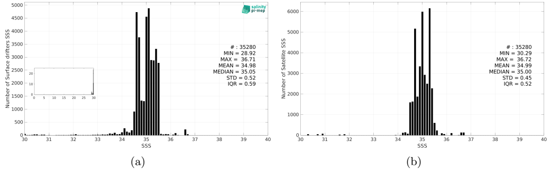
Figure 3: Histograms of SSS from Surface drifters (a) and Aquarius SSS L3 OR v5 - Monthly - Rain mask (NASA-GSFC) (b) considering all match-up pairs per bins of 0.1 over the Tropical Pacific Ocean Pi-MEP region and for the full satellite product period.
