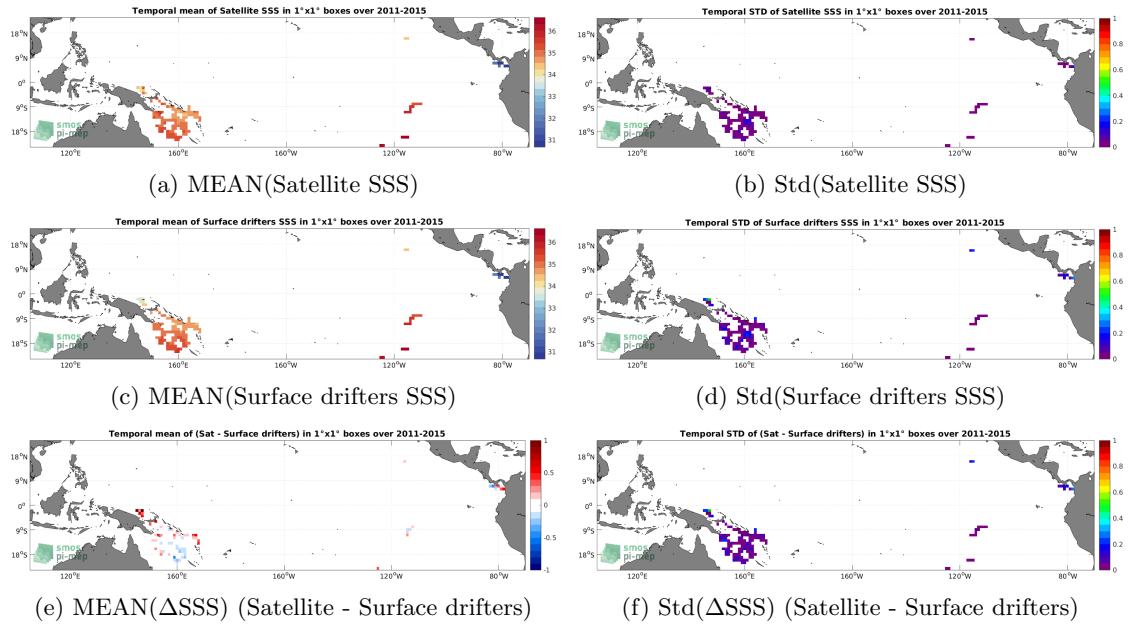
Figure 5: Temporal mean (left) and Std (right) of SSS from Aquarius SSS L3 OR v5 - Monthly - Rain mask (NASA-GSFC) (top), Surface drifters (middle), and of \Delta SSS (Satellite - Surface drifters). Only match-up pairs are used to generate these maps.
