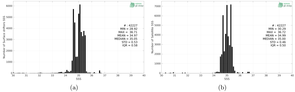
Figure 2: Histograms of SSS from Surface drifters (a) and Aquarius SSS L3 OR v5 - Monthly - Rain mask (NASA-GSFC) (b) considering all match-up pairs per bins of 0.1 over the Tropical Pacific Ocean Pi-MEP region and for the full satellite product period.
