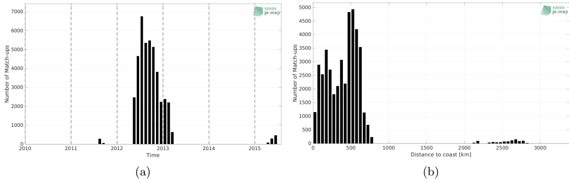
Figure 1: Number of match-ups between Surface drifters and Aquarius SSS L3 OR v5 - Monthly - Rain mask (NASA-GSFC) SSS as a function of time (a) and as function of the distance to coast (b) over the Tropical Pacific Ocean Pi-MEP region and for the full satellite product period.
