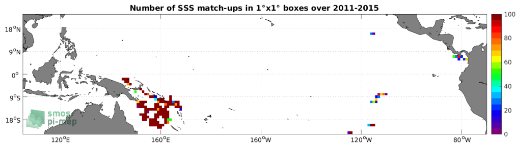
Figure 3: Number of SSS match-ups between Surface drifters SSS and the Aquarius SSS L3 OR v5 - Monthly - Rain mask (NASA-GSFC) SSS product for the Tropical Pacific Ocean Pi-MEP region over 1^\circ \times 1^\circ boxes and for the full satellite product period.
