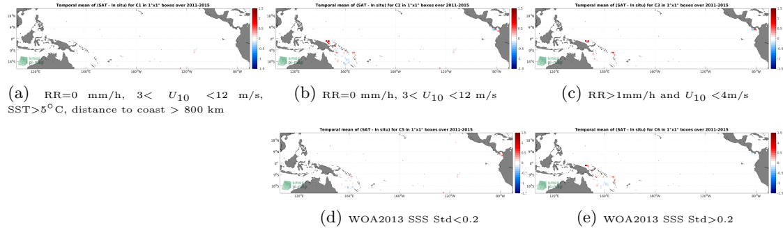
Figure 11: Temporal mean gridded over spatial boxes of size 1^{\circ}\times 1^{\circ} of \Delta\text{SSS} (Aquarius SSS L3 OR v5 - Monthly - Rain mask (NASA-GSFC) - Surface drifters) for 5 different subdatasets corresponding to:RR=0 mm/h, 3 < U_{10} < 12 m/s, SST > 5^{\circ}\text{C} , distance to coast > 800 km (a), RR=0 mm/h, 3 < U_{10} < 12 m/s (b), RR > 1 mm/h and U_{10} < 4 m/s (c), WOA2013 SSS Std < 0.2 (d), WOA2013 SSS Std > 0.2 (e).
