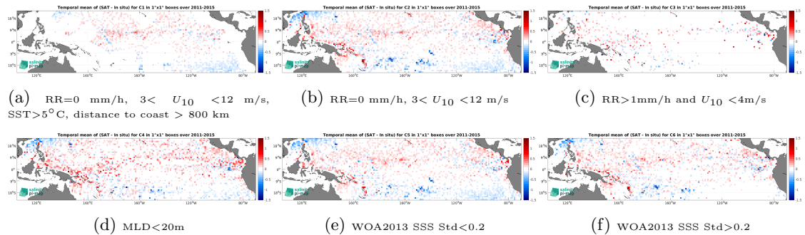
Figure 14: Temporal mean gridded over spatial boxes of size 1^\circ \times 1^\circ of \Delta SSS (Aquarius SSS L3 OR v5 - Monthly - Rain mask (NASA-GSFC) - Argo) for 6 different subdatasets corresponding to:RR=0 mm/h, 3 < U_{10} < 12 m/s, SST >5^\circ C, distance to coast > 800 km (a), RR=0 mm/h, 3 < U_{10} < 12 m/s (b), RR >1 mm/h and U_{10} < 4 m/s (c),MLD <20 m (d),WOA2013 SSS Std <0.2 (e),WOA2013 SSS Std >0.2 (f).
