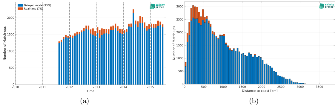
Figure 2: Number of match-ups between Argo and Aquarius SSS L3 OR v5 - Monthly - Rain mask (NASA-GSFC) SSS as a function of time (a) and as function of the distance to coast (b) over the Tropical Pacific Ocean Pi-MEP region and for the full satellite product period.
