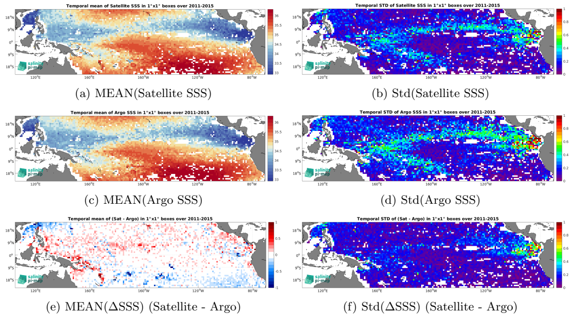
Figure 7: Temporal mean (left) and Std (right) of SSS from Aquarius SSS L3 OR v5 - Monthly - Rain mask (NASA-GSFC) (top), Argo (middle), and of \Delta SSS (Satellite - Argo). Only match-up pairs are used to generate these maps.
