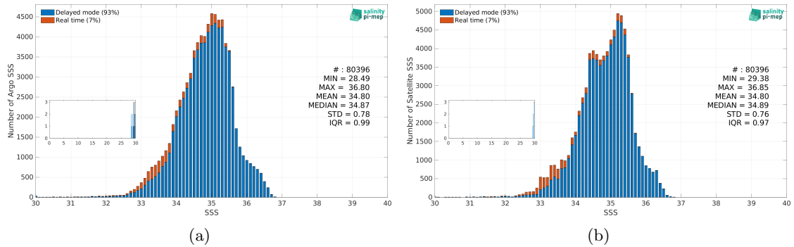
Figure 3: Histograms of SSS from Argo (a) and Aquarius SSS L3 OR v5 - Monthly - Rain mask (NASA-GSFC) (b) considering all match-up pairs per bins of 0.1 over the Tropical Pacific Ocean Pi-MEP region and for the full satellite product period.
