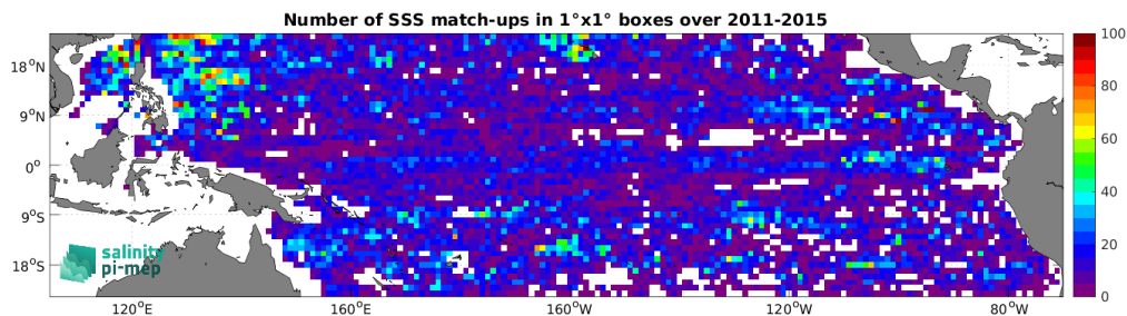
Figure 5: Number of SSS match-ups between Argo SSS and the Aquarius SSS L3 OR v5 - Monthly - Rain mask (NASA-GSFC) SSS product for the Tropical Pacific Ocean Pi-MEP region over 1^\circ \times 1^\circ boxes and for the full satellite product period.
