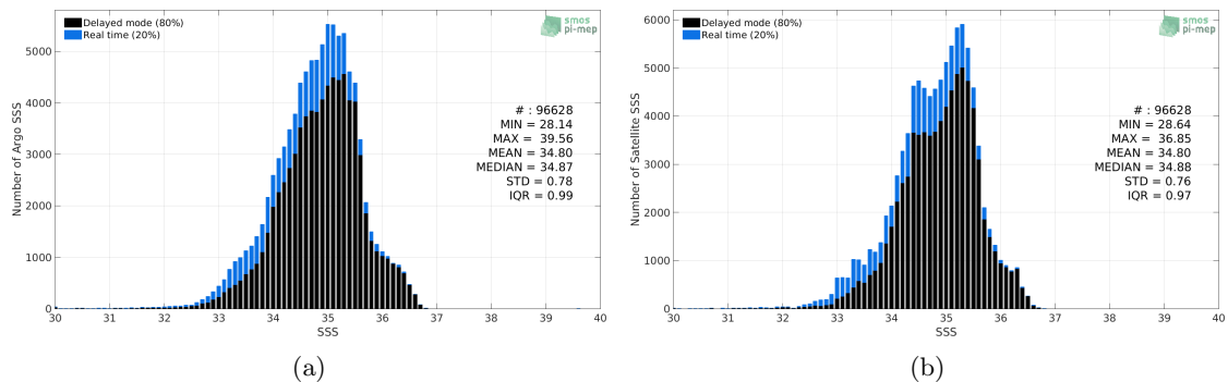
Figure 2: Histograms of SSS from Argo (a) and Aquarius-L3-OR-V5-MONTHLY-RAIN-MASK-1DEG (b) considering all match-up pairs per bins of 0.1 over the Tropical Pacific Ocean Pi-MEP region and for the full satellite product period.
