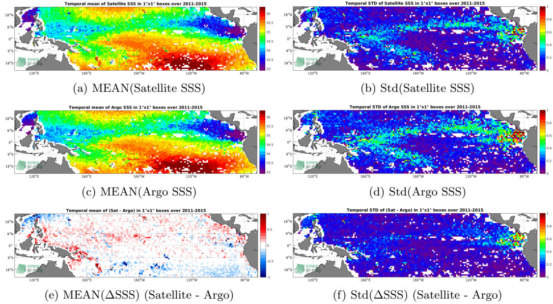
Figure 6: Temporal mean (left) and Std (right) of SSS from Aquarius-L3-OR-V5-MONTHLY-RAIN-MASK-1DEG (top), Argo (middle), and of \Delta SSS (Satellite - Argo). Only match-up pairs are used to generate these maps.
