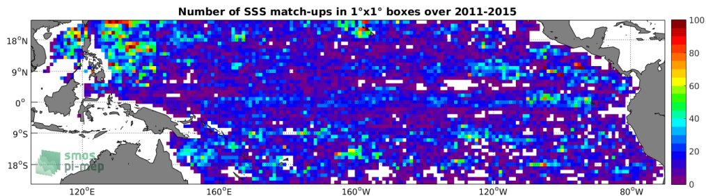
Figure 4: Number of SSS match-ups between Argo SSS and the Aquarius-L3-OR-V5-MONTHLY-RAIN-MASK-1DEG SSS product for the Tropical Pacific Ocean Pi-MEP region over 1^{\circ} \times 1^{\circ} boxes and for the full satellite product period.
