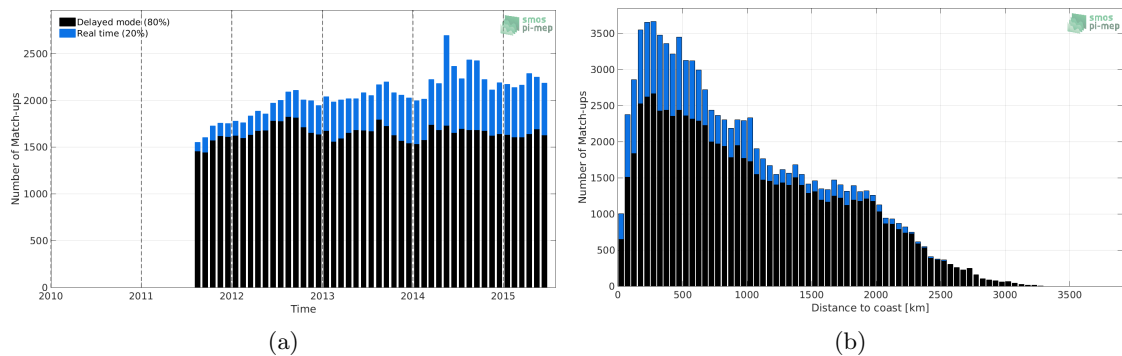
Figure 1: Number of match-ups between Argo and Aquarius-L3-OR-V5-MONTHLY-RAIN-MASK-1DEG SSS as a function of time (a) and as function of the distance to coast (b) over the Tropical Pacific Ocean Pi-MEP region and for the full satellite product period.
