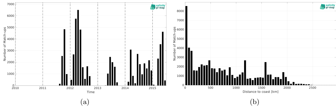
Figure 1: Number of match-ups between TSG (SAMOS) and Aquarius SSS L3 CAP v5 - 7-Day running (JPL) SSS as a function of time (a) and as function of the distance to coast (b) over the Tropical Pacific Ocean Pi-MEP region and for the full satellite product period.
