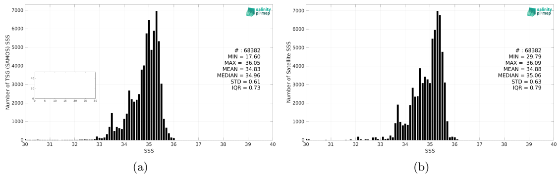
Figure 2: Histograms of SSS from TSG (SAMOS) (a) and Aquarius SSS L3 CAP v5 - 7-Day running (JPL) (b) considering all match-up pairs per bins of 0.1 over the Tropical Pacific Ocean Pi-MEP region and for the full satellite product period.
