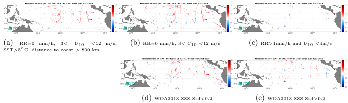
Figure 12: Temporal mean gridded over spatial boxes of size 1^\circ \times 1^\circ of \Delta\text{SSS} (Aquarius SSS L3 CAP v5 - 7-Day running (JPL) - TSG (SAMOS)) for 5 different subdatasets corresponding to:RR=0 mm/h, 3 < U_{10} < 12 m/s, SST >5^\circ\text{C} , distance to coast > 800 km (a), RR=0 mm/h, 3 < U_{10} < 12 m/s (b), RR >1 mm/h and U_{10} < 4 m/s (c), WOA2013 SSS Std <0.2 (d), WOA2013 SSS Std >0.2 (e).
