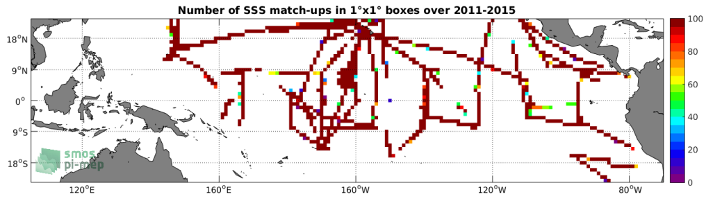
Figure 4: Number of SSS match-ups between TSG-SAMOS SSS and the Aquarius-L3-JPL-V5-7DAY-RUNNING SSS product for the Tropical Pacific Ocean Pi-MEP region over 1^\circ \times 1^\circ boxes and for the full satellite product period.
