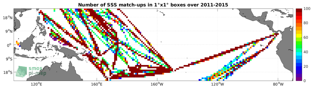
Figure 4: Number of SSS match-ups between TSG (LEGOS-DM) SSS and the Aquarius SSS L3 CAP v5 - 7-Day running (JPL) SSS product for the Tropical Pacific Ocean Pi-MEP region over 1^\circ \times 1^\circ boxes and for the full satellite product period.
