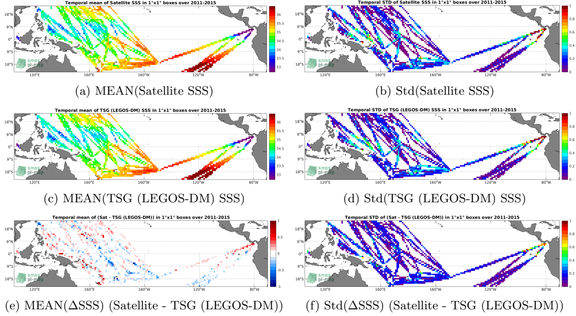
Figure 6: Temporal mean (left) and Std (right) of SSS from Aquarius SSS L3 CAP v5 - 7-Day running (JPL) (top), TSG (LEGOS-DM) (middle), and of \Delta SSS (Satellite - TSG (LEGOS-DM)). Only match-up pairs are used to generate these maps.
