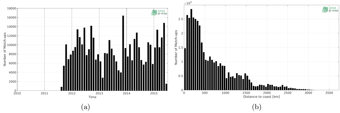
Figure 1: Number of match-ups between TSG (LEGOS-DM) and Aquarius SSS L3 CAP v5 - 7-Day running (JPL) SSS as a function of time (a) and as function of the distance to coast (b) over the Tropical Pacific Ocean Pi-MEP region and for the full satellite product period.
