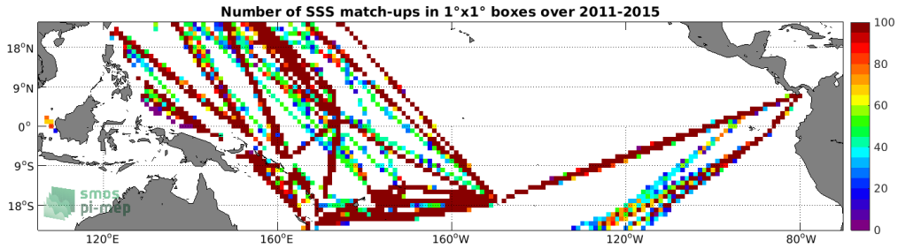
Figure 4: Number of SSS match-ups between TSG (LEGOS-DM) SSS and the Aquarius SSS L3 CAP v5 - 7-Day running (JPL) SSS product for the Tropical Pacific Ocean Pi-MEP region over 1^\circ \times 1^\circ boxes and for the full satellite product period.
