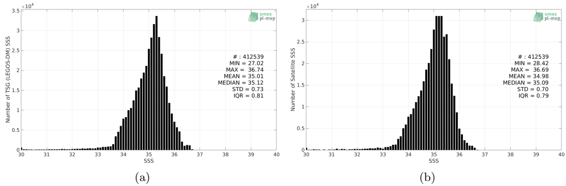
Figure 2: Histograms of SSS from TSG (LEGOS-DM) (a) and Aquarius SSS L3 CAP v5 - 7-Day running (JPL) (b) considering all match-up pairs per bins of 0.1 over the Tropical Pacific Ocean Pi-MEP region and for the full satellite product period.
