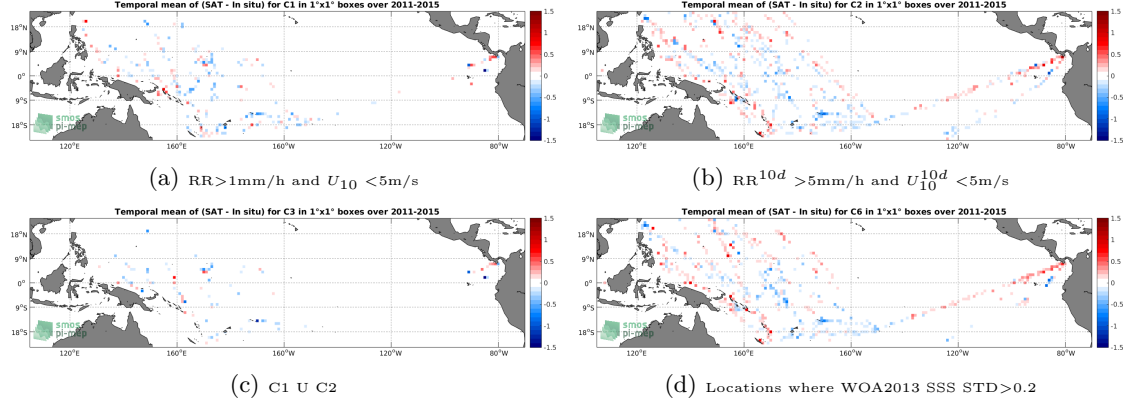
Figure 12: Temporal mean gridded over spatial boxes of size 1^\circ \times 1^\circ of \Delta SSS (Aquarius-L3-JPL-V5-7DAY-RUNNING - TSG-LEGOS-DM) for 4 different subdatasets corresponding to: RR > 1\text{mm/h} and U_{10} < 5\text{m/s} (a), RR^{10d} > 5\text{mm/h} and U_{10}^{10d} < 5\text{m/s} (b), C1 U C2 (c), Locations where WOA2013 SSS STD > 0.2 (d).
