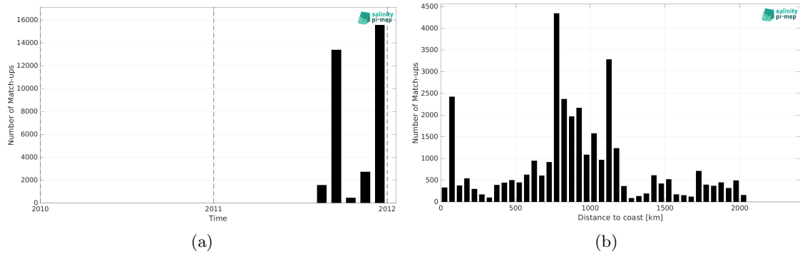
Figure 2: Number of match-ups between TSG (GOSUD-Sailing-ship) and Aquarius SSS L3 CAP v5 - 7-Day running (JPL) SSS as a function of time (a) and as function of the distance to coast (b) over the Tropical Pacific Ocean Pi-MEP region and for the full satellite product period.
