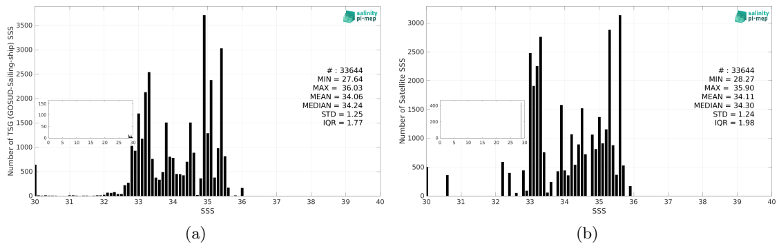
Figure 3: Histograms of SSS from TSG (GOSUD-Sailing-ship) (a) and Aquarius SSS L3 CAP v5 - 7-Day running (JPL) (b) considering all match-up pairs per bins of 0.1 over the Tropical Pacific Ocean Pi-MEP region and for the full satellite product period.
