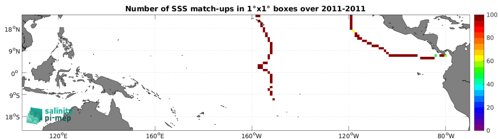
Figure 5: Number of SSS match-ups between TSG (GOSUD-Sailing-ship) SSS and the Aquarius SSS L3 CAP v5 - 7-Day running (JPL) SSS product for the Tropical Pacific Ocean Pi-MEP region over 1^\circ \times 1^\circ boxes and for the full satellite product period.
