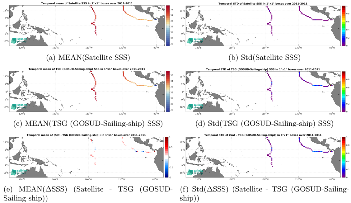
Figure 7: Temporal mean (left) and Std (right) of SSS from Aquarius SSS L3 CAP v5 - 7-Day running (JPL) (top), TSG (GOSUD-Sailing-ship) (middle), and of \Delta SSS (Satellite - TSG (GOSUD-Sailing-ship)). Only match-up pairs are used to generate these maps.
