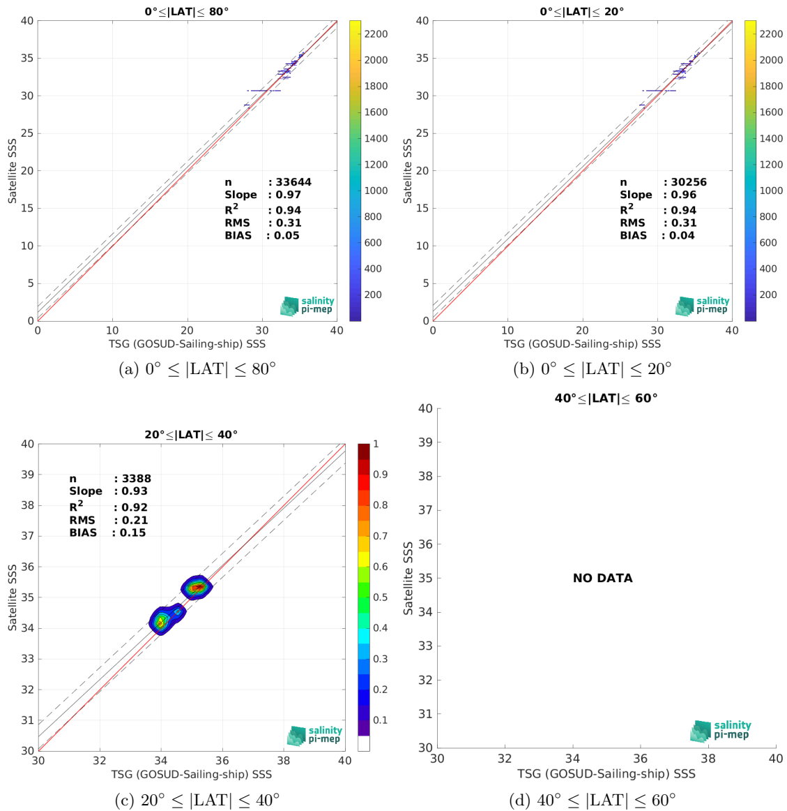
Figure 10: Contour maps of the concentration of Aquarius SSS L3 CAP v5 - 7-Day running (JPL) SSS (y-axis) versus TSG (GOSUD-Sailing-ship) SSS (x-axis) at match-up pairs for different latitude bands. For each plot, the red line shows x=y . The black thin and dashed lines indicate a linear fit through the data cloud and the \pm 95\% confidence levels, respectively. The number match-up pairs n , the slope and R^2 coefficient of the linear fit, the root mean square (RMS) and the mean bias between satellite and in situ data are indicated for each latitude band in each plots.
