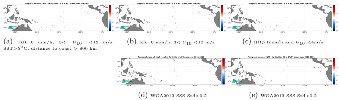
Figure 12: Temporal mean gridded over spatial boxes of size 1^{\circ}\times 1^{\circ} of \Delta SSS (Aquarius SSS L3 CAP v5 - 7-Day running (JPL) - TSG (GOSUD-Sailing-ship)) for 5 different subdatasets corresponding to: RR=0 mm/h, 3 < U_{10} < 12 m/s, SST >5^{\circ}\text{C} , distance to coast > 800 km (a), RR=0 mm/h, 3 < U_{10} < 12 m/s (b), RR >1 mm/h and U_{10} < 4 m/s (c), WOA2013 SSS Std <0.2 (d), WOA2013 SSS Std >0.2 (e).
