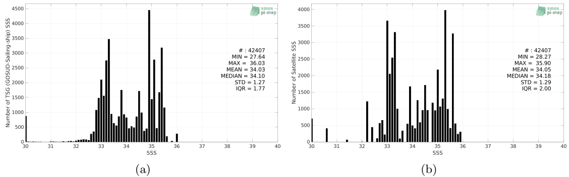
Figure 2: Histograms of SSS from TSG (GOSUD-Sailing-ship) (a) and Aquarius SSS L3 CAP v5 - 7-Day running (JPL) (b) considering all match-up pairs per bins of 0.1 over the Tropical Pacific Ocean Pi-MEP region and for the full satellite product period.
