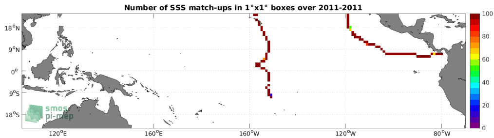
Figure 4: Number of SSS match-ups between TSG (GOSUD-Sailing-ship) SSS and the Aquarius SSS L3 CAP v5 - 7-Day running (JPL) SSS product for the Tropical Pacific Ocean Pi-MEP region over 1^\circ \times 1^\circ boxes and for the full satellite product period.
