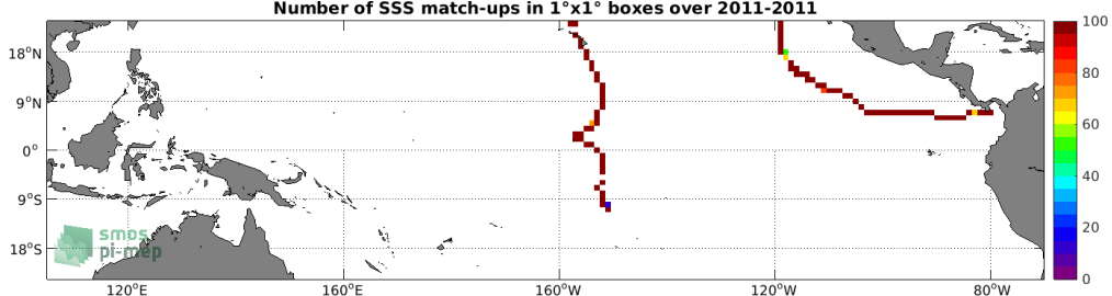
Figure 4: Number of SSS match-ups between TSG (GOSUD-Sailing-ship) SSS and the Aquarius SSS L3 CAP v5 - 7-Day running (JPL) SSS product for the Tropical Pacific Ocean Pi-MEP region over 1^\circ \times 1^\circ boxes and for the full satellite product period.
