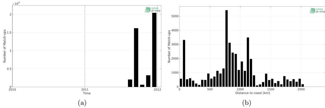
Figure 1: Number of match-ups between TSG (GOSUD-Sailing-ship) and Aquarius SSS L3 CAP v5 - 7-Day running (JPL) SSS as a function of time (a) and as function of the distance to coast (b) over the Tropical Pacific Ocean Pi-MEP region and for the full satellite product period.
