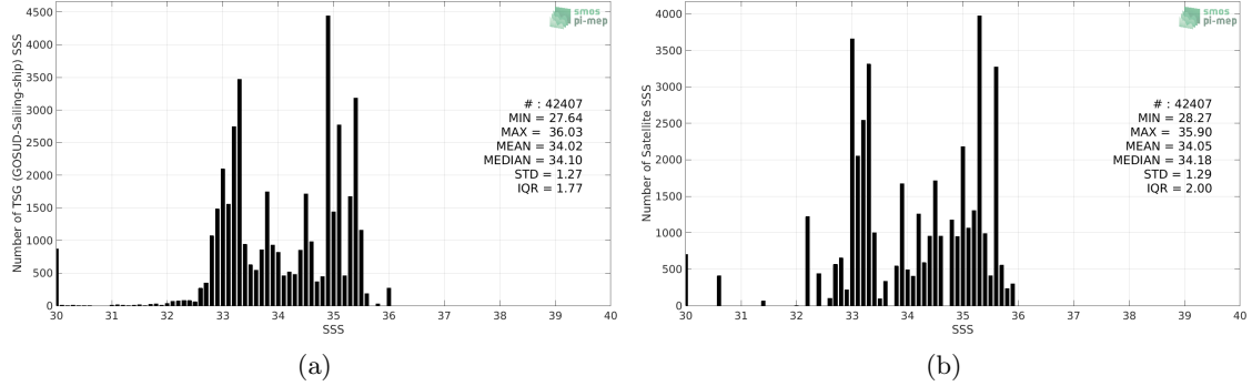
Figure 2: Histograms of SSS from TSG (GOSUD-Sailing-ship) (a) and Aquarius SSS L3 CAP v5 - 7-Day running (JPL) (b) considering all match-up pairs per bins of 0.1 over the Tropical Pacific Ocean Pi-MEP region and for the full satellite product period.
