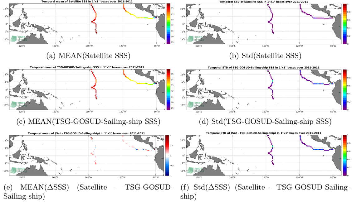
Figure 6: Temporal mean (left) and Std (right) of SSS from Aquarius-L3-JPL-V5-7DAY-RUNNING (top), TSG-GOSUD-Sailing-ship (middle), and of \Delta SSS (Satellite - TSG-GOSUD-Sailing-ship). Only match-up pairs are used to generate these maps.
