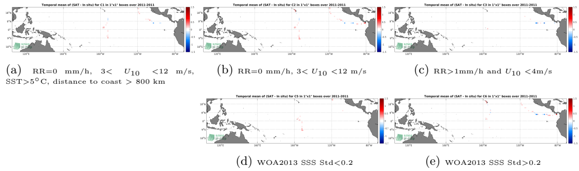
Figure 12: Temporal mean gridded over spatial boxes of size 1^\circ \times 1^\circ of \Delta SSS (Aquarius-L3-JPL-V5-7DAY-RUNNING - TSG-GOSUD-Sailing-ship) for 5 different subdatasets corresponding to: RR=0 mm/h, 3 < U_{10} < 12 m/s, SST > 5^\circ C , distance to coast > 800 km (a), RR=0 mm/h, 3 < U_{10} < 12 m/s (b), RR > 1 mm/h and U_{10} < 4 m/s (c), WOA2013 SSS Std < 0.2 (d), WOA2013 SSS Std > 0.2 (e).
