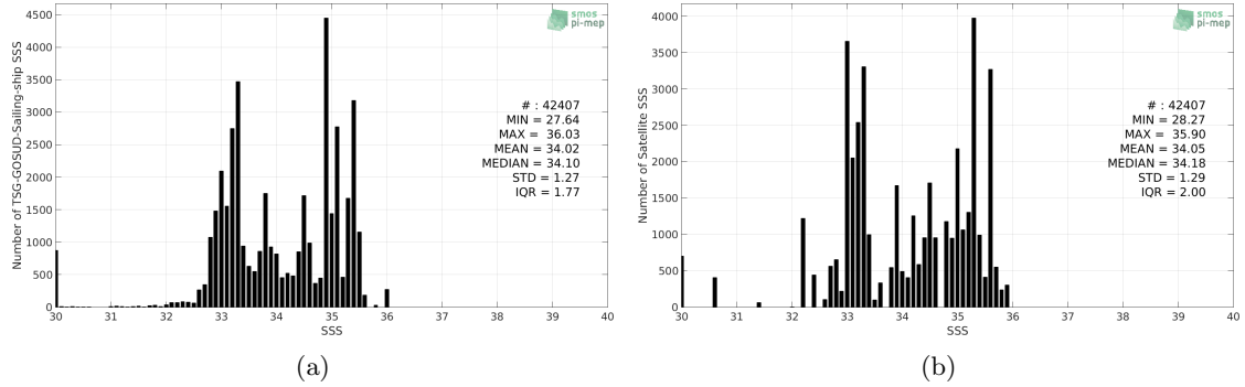
Figure 2: Histograms of SSS from TSG-GOSUD-Sailing-ship (a) and Aquarius-L3-JPL-V5-7DAY-RUNNING (b) considering all match-up pairs per bins of 0.1 over the Tropical Pacific Ocean Pi-MEP region and for the full satellite product period.
