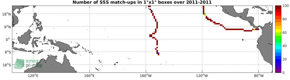
Figure 4: Number of SSS match-ups between TSG-GOSUD-Sailing-ship SSS and the Aquarius-L3-JPL-V5-7DAY-RUNNING SSS product for the Tropical Pacific Ocean Pi-MEP region over 1^\circ \times 1^\circ boxes and for the full satellite product period.
