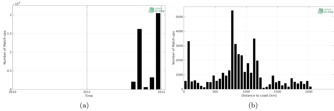
Figure 1: Number of match-ups between TSG-GOSUD-Sailing-ship and Aquarius-L3-JPL-V5-7DAY-RUNNING SSS as a function of time (a) and as function of the distance to coast (b) over the Tropical Pacific Ocean Pi-MEP region and for the full satellite product period.
