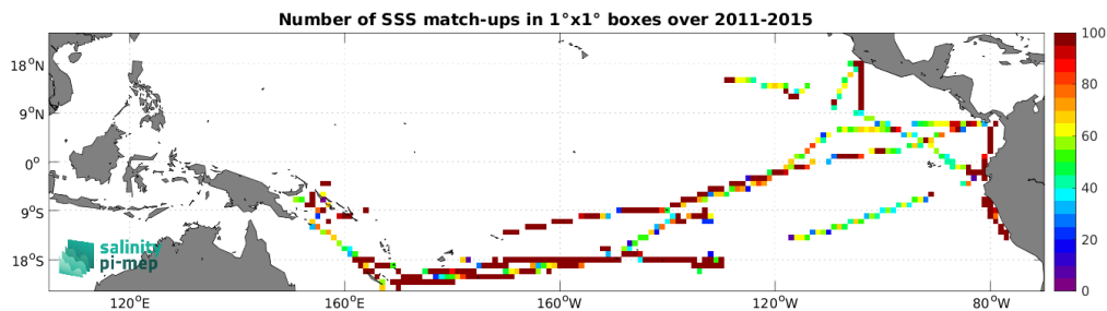
Figure 5: Number of SSS match-ups between TSG (GOSUD-Research-vessel) SSS and the Aquarius SSS L3 CAP v5 - 7-Day running (JPL) SSS product for the Tropical Pacific Ocean Pi-MEP region over 1^\circ \times 1^\circ boxes and for the full satellite product period.
