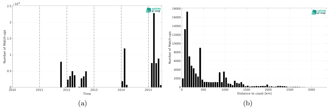
Figure 2: Number of match-ups between TSG (GOSUD-Research-vessel) and Aquarius SSS L3 CAP v5 - 7-Day running (JPL) SSS as a function of time (a) and as function of the distance to coast (b) over the Tropical Pacific Ocean Pi-MEP region and for the full satellite product period.
