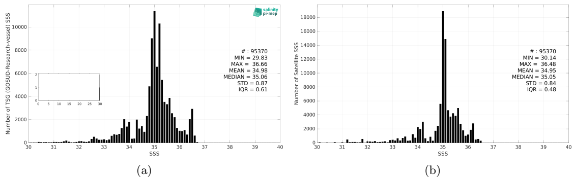
Figure 3: Histograms of SSS from TSG (GOSUD-Research-vessel) (a) and Aquarius SSS L3 CAP v5 - 7-Day running (JPL) (b) considering all match-up pairs per bins of 0.1 over the Tropical Pacific Ocean Pi-MEP region and for the full satellite product period.
