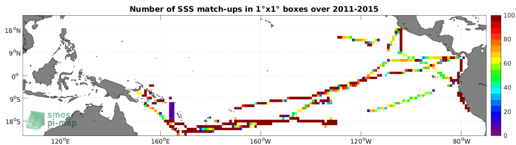
Figure 4: Number of SSS match-ups between TSG (GOSUD-Research-vessel) SSS and the Aquarius SSS L3 CAP v5 - 7-Day running (JPL) SSS product for the Tropical Pacific Ocean Pi-MEP region over 1^\circ \times 1^\circ boxes and for the full satellite product period.
