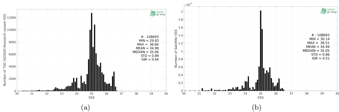
Figure 2: Histograms of SSS from TSG (GOSUD-Research-vessel) (a) and Aquarius SSS L3 CAP v5 - 7-Day running (JPL) (b) considering all match-up pairs per bins of 0.1 over the Tropical Pacific Ocean Pi-MEP region and for the full satellite product period.
