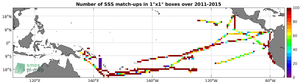
Figure 4: Number of SSS match-ups between TSG (GOSUD-Research-vessel) SSS and the Aquarius SSS L3 CAP v5 - 7-Day running (JPL) SSS product for the Tropical Pacific Ocean Pi-MEP region over 1^\circ \times 1^\circ boxes and for the full satellite product period.
