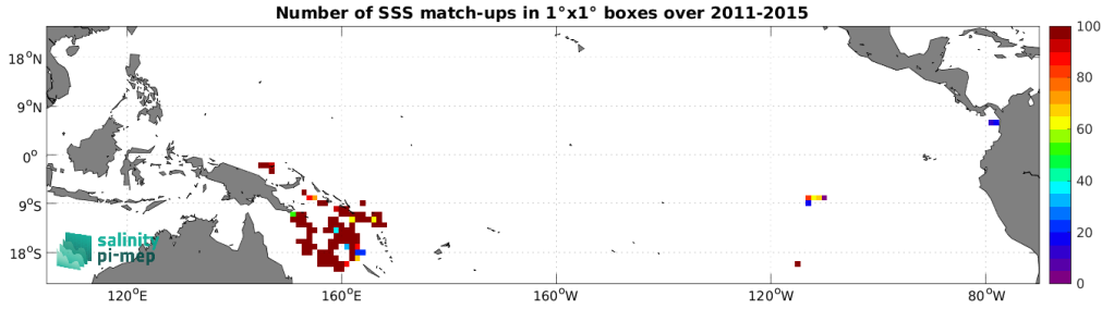
Figure 4: Number of SSS match-ups between Surface drifters SSS and the Aquarius SSS L3 CAP v5 - 7-Day running (JPL) SSS product for the Tropical Pacific Ocean Pi-MEP region over 1^\circ \times 1^\circ boxes and for the full satellite product period.
