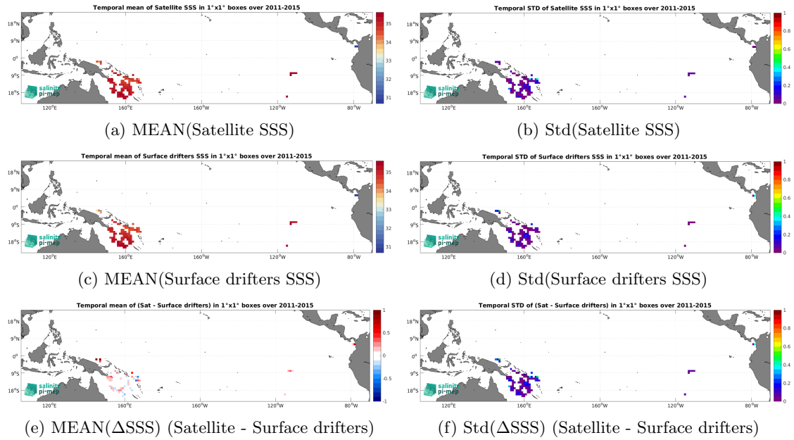
Figure 6: Temporal mean (left) and Std (right) of SSS from Aquarius SSS L3 CAP v5 - 7-Day running (JPL) (top), Surface drifters (middle), and of \Delta SSS (Satellite - Surface drifters). Only match-up pairs are used to generate these maps.
