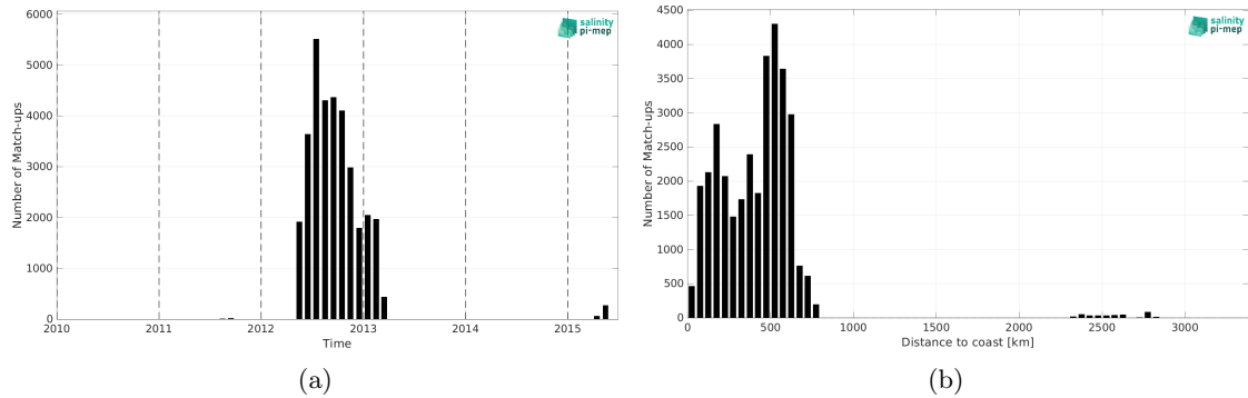
Figure 2: Number of match-ups between Surface drifters and Aquarius SSS L3 CAP v5 - 7-Day running (JPL) SSS as a function of time (a) and as function of the distance to coast (b) over the Tropical Pacific Ocean Pi-MEP region and for the full satellite product period.
