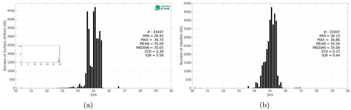
Figure 3: Histograms of SSS from Surface drifters (a) and Aquarius SSS L3 CAP v5 - 7-Day running (JPL) (b) considering all match-up pairs per bins of 0.1 over the Tropical Pacific Ocean Pi-MEP region and for the full satellite product period.
