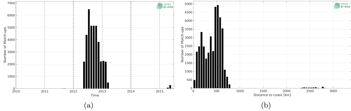
Figure 1: Number of match-ups between Surface drifters and Aquarius SSS L3 CAP v5 - 7-Day running (JPL) SSS as a function of time (a) and as function of the distance to coast (b) over the Tropical Pacific Ocean Pi-MEP region and for the full satellite product period.
