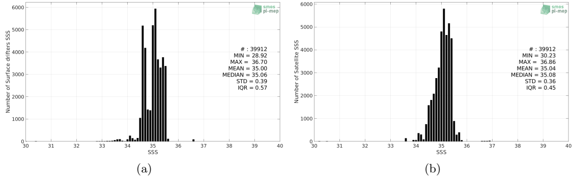
Figure 2: Histograms of SSS from Surface drifters (a) and Aquarius SSS L3 CAP v5 - 7-Day running (JPL) (b) considering all match-up pairs per bins of 0.1 over the Tropical Pacific Ocean Pi-MEP region and for the full satellite product period.
