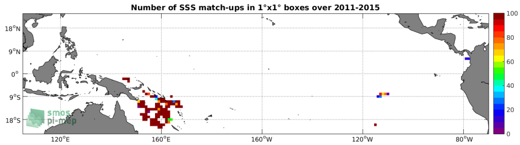
Figure 3: Number of SSS match-ups between Surface drifters SSS and the Aquarius-L3-JPL-V5-7DAY-RUNNING SSS product for the Tropical Pacific Ocean Pi-MEP region over 1°x1° boxes and for the full satellite product period.
