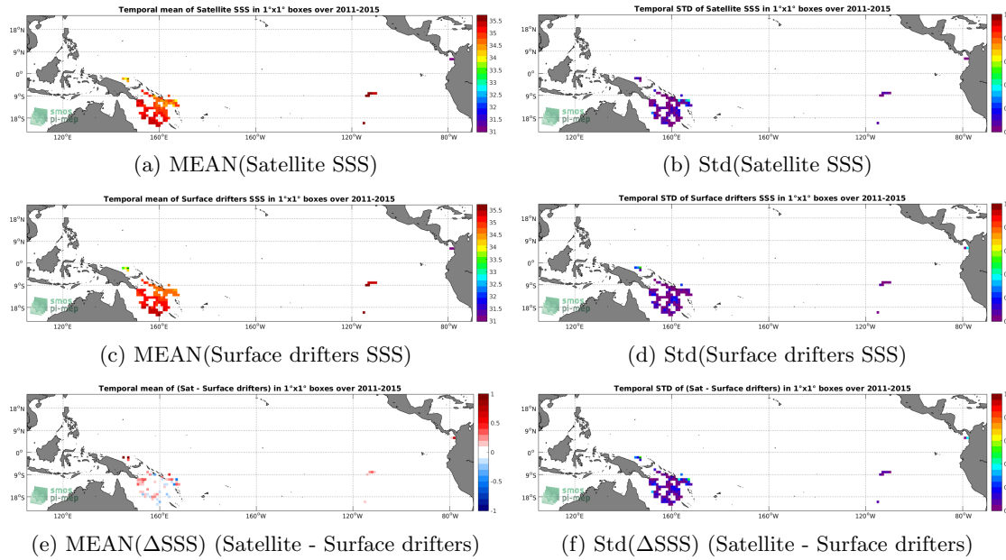
Figure 5: Temporal mean (left) and Std (right) of SSS from Aquarius-L3-JPL-V5-7DAY-RUNNING (top), Surface drifters (middle), and of \Delta SSS (Satellite - Surface drifters). Only match-up pairs are used to generate these maps.
