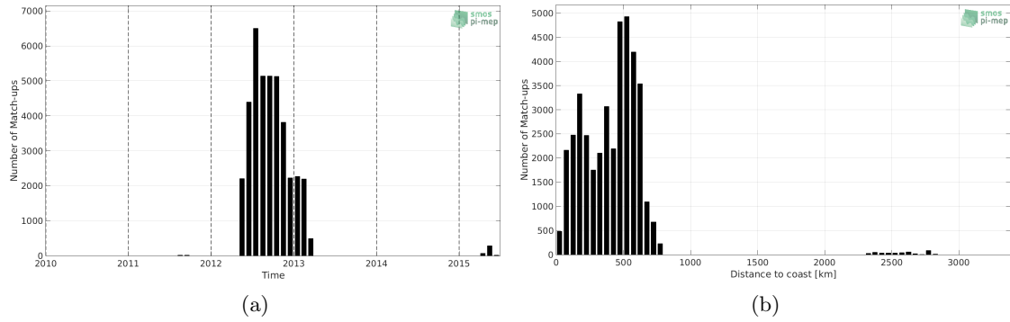
Figure 1: Number of match-ups between Surface drifters and Aquarius-L3-JPL-V5-7DAY-RUNNING SSS as a function of time (a) and as function of the distance to coast (b) over the Tropical Pacific Ocean Pi-MEP region and for the full satellite product period.
