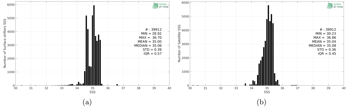
Figure 2: Histograms of SSS from Surface drifters (a) and Aquarius-L3-JPL-V5-7DAY-RUNNING (b) considering all match-up pairs per bins of 0.1 over the Tropical Pacific Ocean Pi-MEP region and for the full satellite product period.
