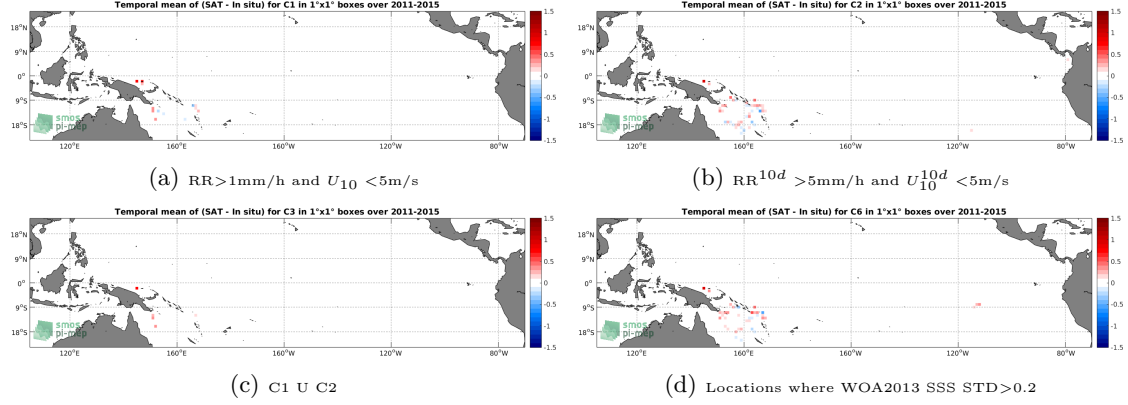
Figure 11: Temporal mean gridded over spatial boxes of size 1^\circ \times 1^\circ of \Delta SSS (Aquarius-L3-JPL-V5-7DAY-RUNNING - Surface drifters) for 4 different subdatasets corresponding to: RR > 1\text{mm/h} and U_{10} < 5\text{m/s} (a), RR^{10d} > 5\text{mm/h} and U_{10}^{10d} < 5\text{m/s} (b), C1 U C2 (c), Locations where WOA2013 SSS STD > 0.2 (d).
