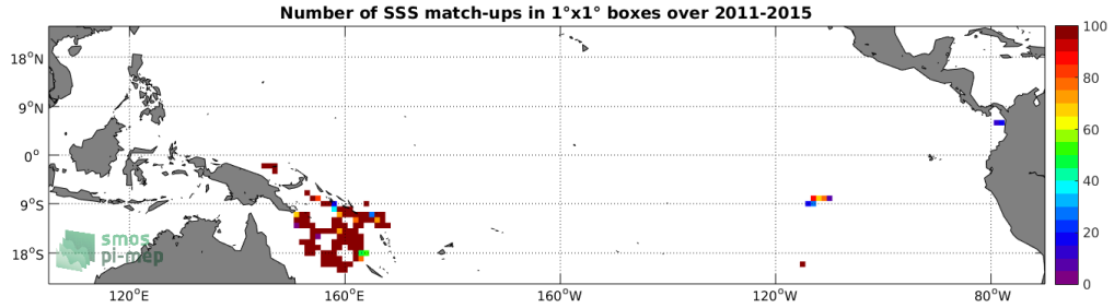
Figure 3: Number of SSS match-ups between Surface drifters SSS and the Aquarius-L3-JPL-V5-7DAY-RUNNING SSS product for the Tropical Pacific Ocean Pi-MEP region over 1^\circ \times 1^\circ boxes and for the full satellite product period.
