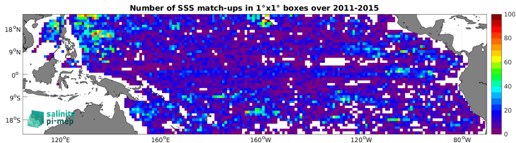
Figure 5: Number of SSS match-ups between Argo SSS and the Aquarius SSS L3 CAP v5 - 7-Day running (JPL) SSS product for the Tropical Pacific Ocean Pi-MEP region over 1^\circ \times 1^\circ boxes and for the full satellite product period.
