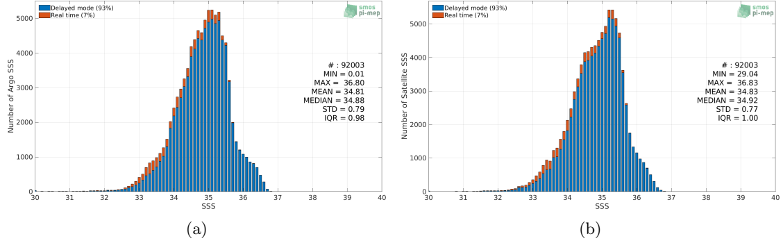
Figure 2: Histograms of SSS from Argo (a) and Aquarius SSS L3 CAP v5 - 7-Day running (JPL) (b) considering all match-up pairs per bins of 0.1 over the Tropical Pacific Ocean Pi-MEP region and for the full satellite product period.
