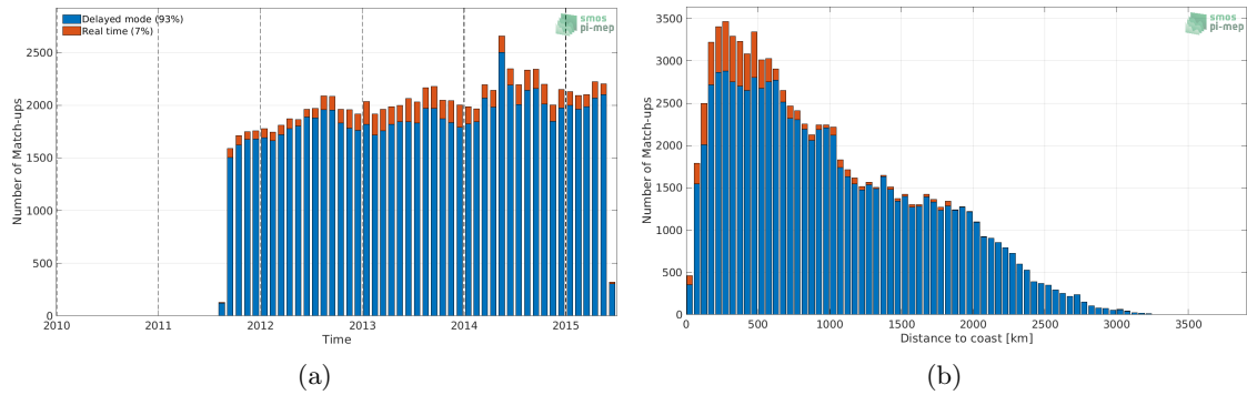
Figure 1: Number of match-ups between Argo and Aquarius SSS L3 CAP v5 - 7-Day running (JPL) SSS as a function of time (a) and as function of the distance to coast (b) over the Tropical Pacific Ocean Pi-MEP region and for the full satellite product period.
