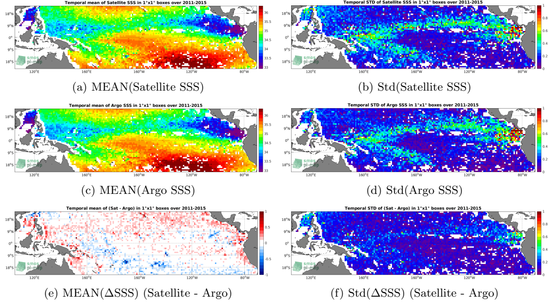
Figure 6: Temporal mean (left) and Std (right) of SSS from Aquarius SSS L3 CAP v5 - 7-Day running (JPL) (top), Argo (middle), and of \Delta SSS (Satellite - Argo). Only match-up pairs are used to generate these maps.
