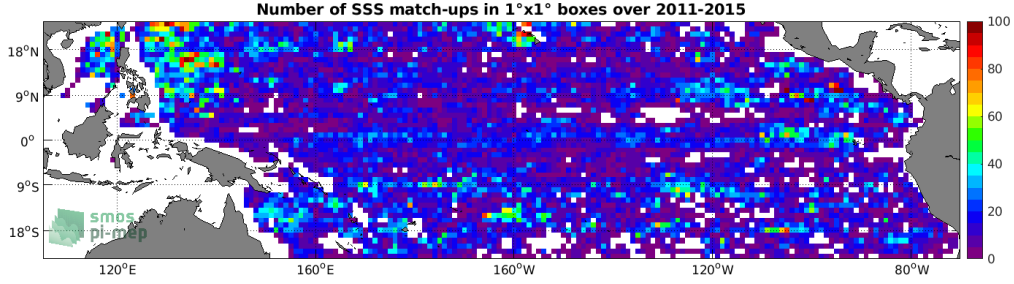
Figure 4: Number of SSS match-ups between Argo SSS and the Aquarius SSS L3 CAP v5 - 7-Day running (JPL) SSS product for the Tropical Pacific Ocean Pi-MEP region over 1^\circ \times 1^\circ boxes and for the full satellite product period.
