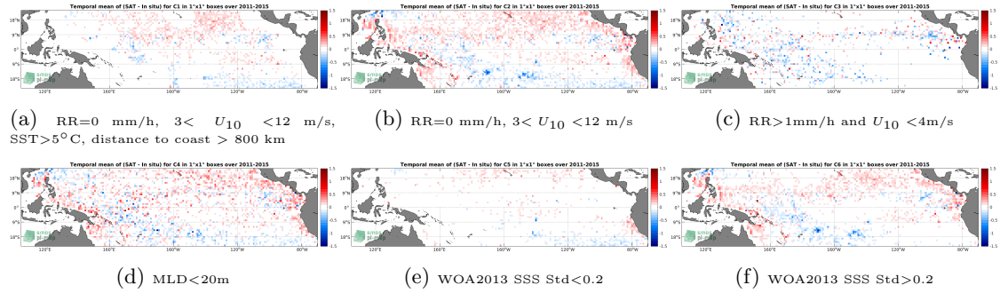
Figure 12: Temporal mean gridded over spatial boxes of size 1^\circ \times 1^\circ of \Delta SSS (Aquarius SSS L3 CAP v5 - 7-Day running (JPL) - Argo) for 6 different subdatasets corresponding to: RR=0 mm/h, 3 < U_{10} < 12 m/s, SST > 5^\circ C , distance to coast > 800 km (a), RR=0 mm/h, 3 < U_{10} < 12 m/s (b), RR > 1 mm/h and U_{10} < 4 m/s (c), MLD < 20 m (d), WOA2013 SSS Std < 0.2 (e), WOA2013 SSS Std > 0.2 (f).
