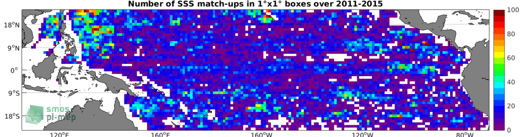
Figure 4: Number of SSS match-ups between Argo SSS and the Aquarius SSS L3 CAP v5 - 7-Day running (JPL) SSS product for the Tropical Pacific Ocean Pi-MEP region over 1^\circ \times 1^\circ boxes and for the full satellite product period.
