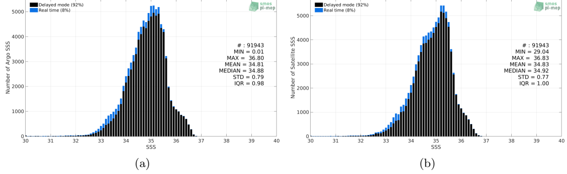
Figure 2: Histograms of SSS from Argo (a) and Aquarius SSS L3 CAP v5 - 7-Day running (JPL) (b) considering all match-up pairs per bins of 0.1 over the Tropical Pacific Ocean Pi-MEP region and for the full satellite product period.
