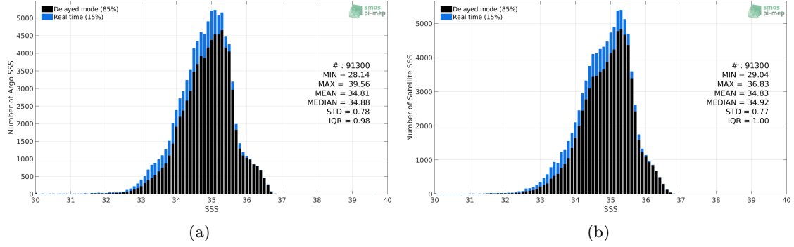
Figure 2: Histograms of SSS from Argo (a) and Aquarius-L3-JPL-V5-7DAY-RUNNING (b) considering all match-up pairs per bins of 0.1 over the Tropical Pacific Ocean Pi-MEP region and for the full satellite product period.
