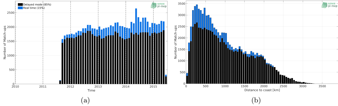
Figure 1: Number of match-ups between Argo and Aquarius-L3-JPL-V5-7DAY-RUNNING SSS as a function of time (a) and as function of the distance to coast (b) over the Tropical Pacific Ocean Pi-MEP region and for the full satellite product period.
