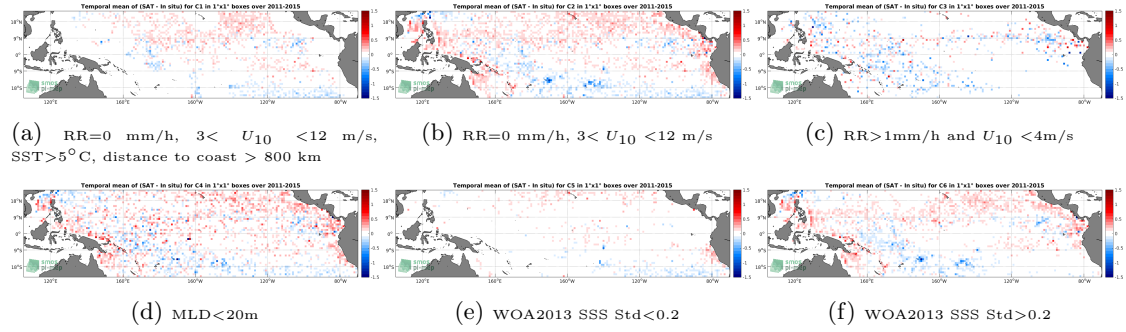
Figure 12: Temporal mean gridded over spatial boxes of size 1^\circ \times 1^\circ of \Delta SSS (Aquarius-L3-JPL-V5-7DAY-RUNNING - Argo) for 6 different subdatasets corresponding to: RR=0 mm/h, 3 < U_{10} < 12 m/s, SST > 5^\circ C , distance to coast > 800 km (a), RR=0 mm/h, 3 < U_{10} < 12 m/s (b), RR > 1 mm/h and U_{10} < 4 m/s (c), MLD < 20 m (d), WOA2013 SSS Std < 0.2 (e), WOA2013 SSS Std > 0.2 (f).
