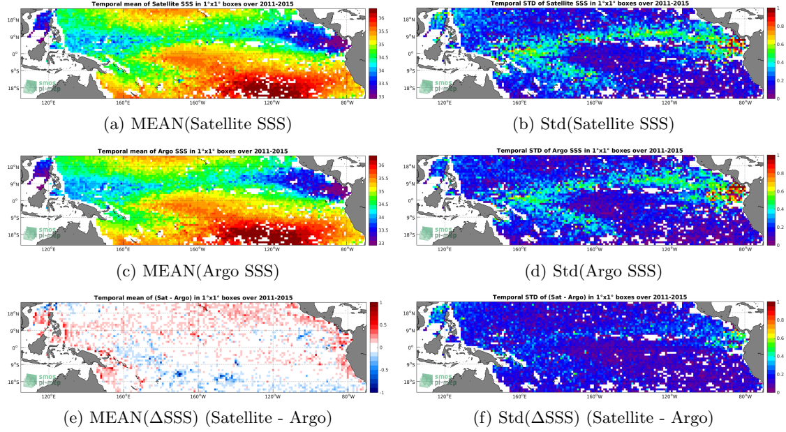
Figure 6: Temporal mean (left) and Std (right) of SSS from Aquarius-L3-JPL-V5-7DAY-RUNNING (top), Argo (middle), and of \Delta SSS (Satellite - Argo). Only match-up pairs are used to generate these maps.
